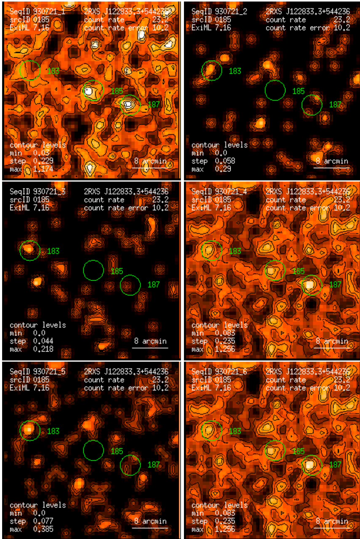
Figure 185: RASS 930721: detection 0185: band rate images, Gaussian filter: (1) PSPC channels 11 – 41, (2) 52 – 90, (3) 91 – 201, (4) 11 – 235, (5) 52 – 201, (6) 11 – 201. Broad band rates in counts/ks. Band rate contour levels in counts/ks/arcmin 2 .
