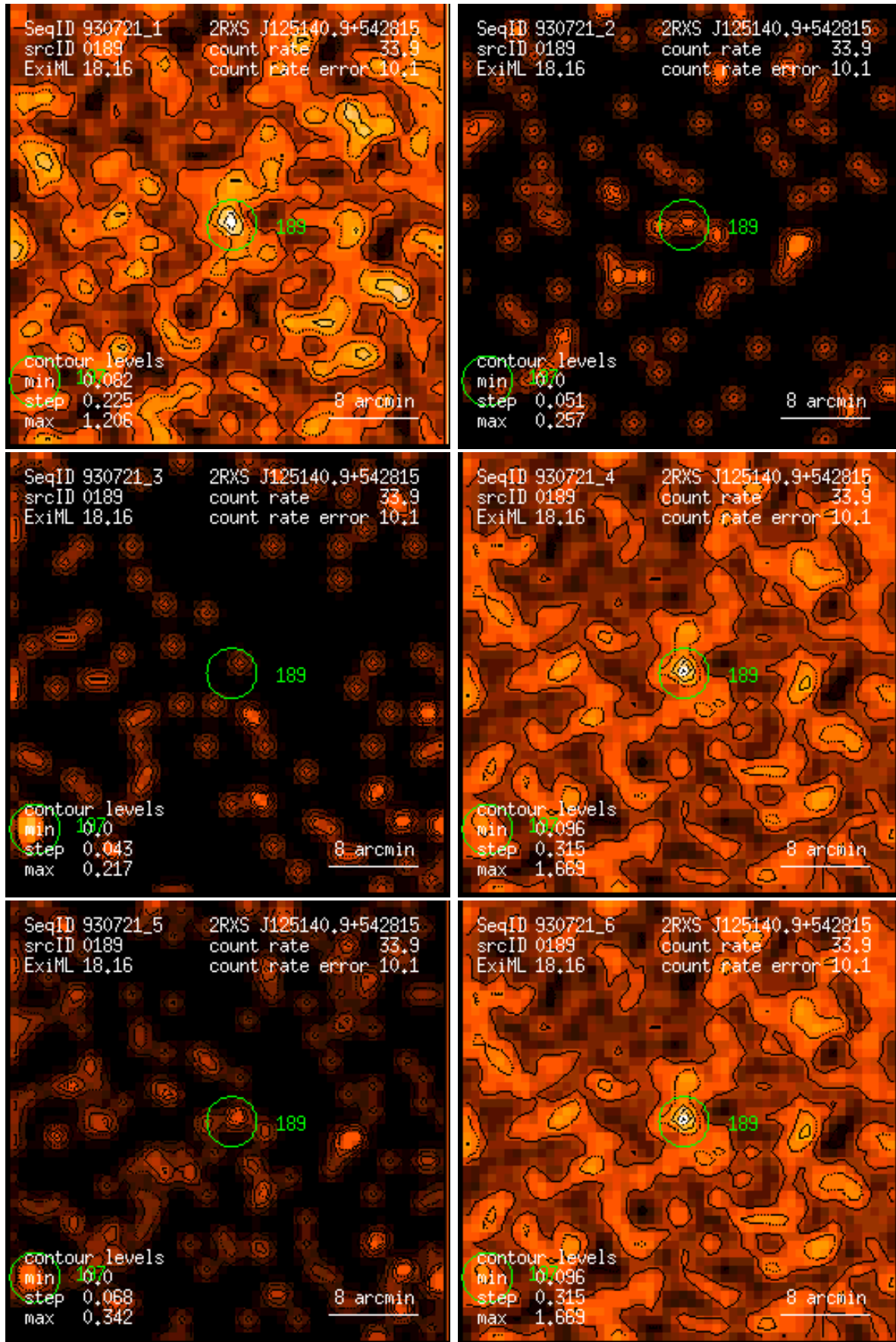
Figure 189: RASS 930721: detection 0189: band rate images, Gaussian filter: (1) PSPC channels 11 – 41, (2) 52 – 90, (3) 91 – 201, (4) 11 – 235, (5) 52 – 201, (6) 11 – 201. Broad band rates in counts/ks. Band rate contour levels in counts/ks/arcmin 2 .
