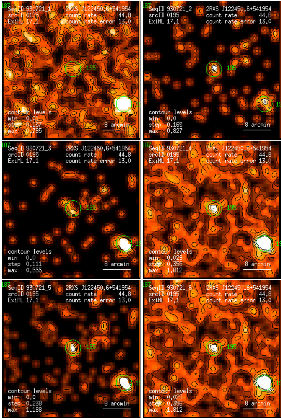
Figure 195: RASS 930721: detection 0195: band rate images, Gaussian filter: (1) PSPC channels 11 – 41, (2) 52 – 90, (3) 91 – 201, (4) 11 – 235, (5) 52 – 201, (6) 11 – 201. Broad band rates in counts/ks. Band rate contour levels in counts/ks/arcmin 2 .
