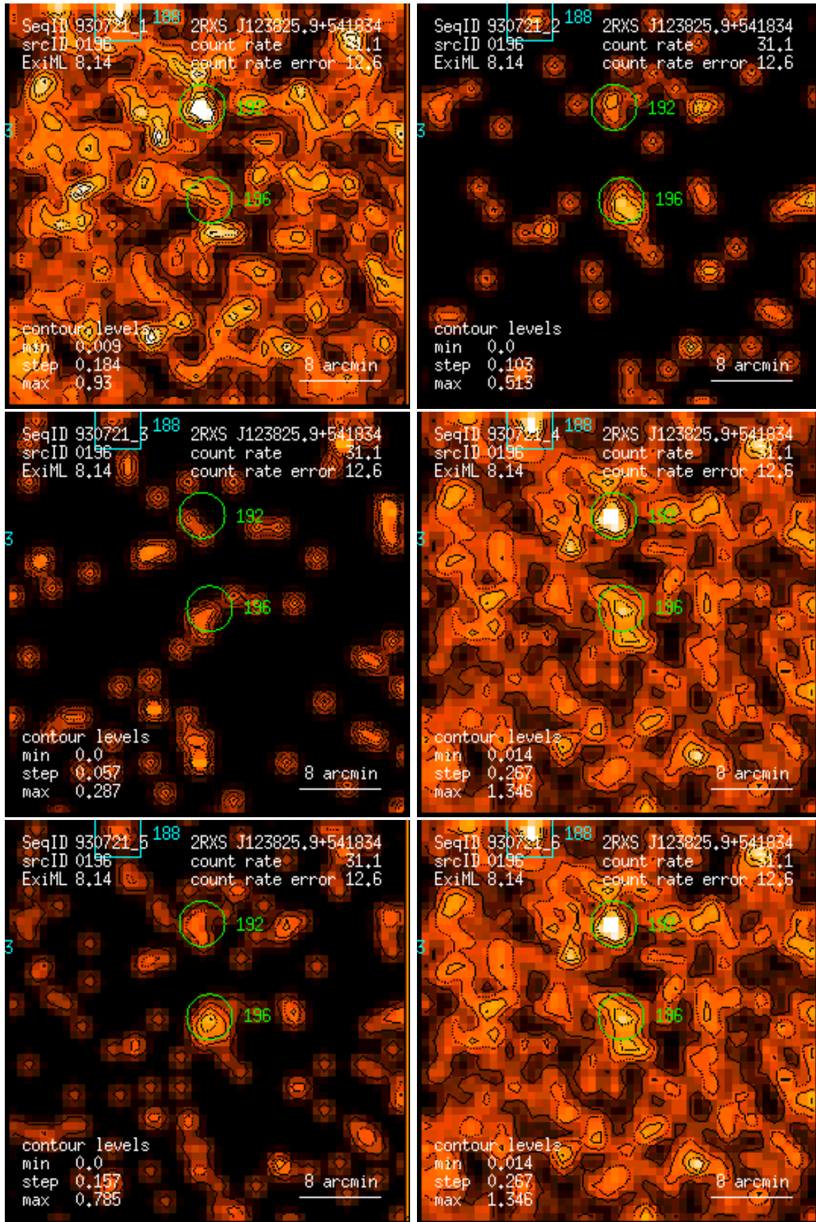
Figure 196: RASS 930721: detection 0196: band rate images, Gaussian filter: (1) PSPC channels 11 – 41, (2) 52 – 90, (3) 91 – 201, (4) 11 – 235, (5) 52 – 201, (6) 11 – 201. Broad band rates in counts/ks. Band rate contour levels in counts/ks/arcmin 2 .
