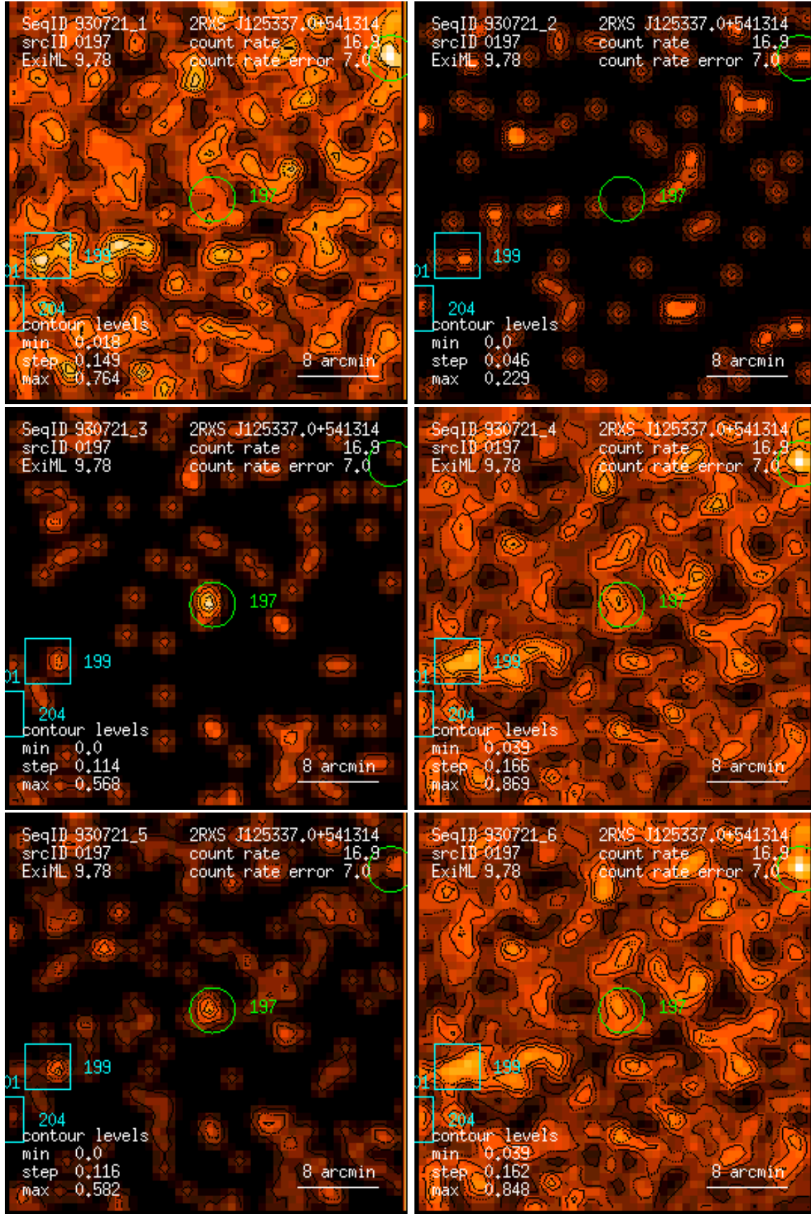
Figure 197: RASS 930721: detection 0197: band rate images, Gaussian filter: (1) PSPC channels 11 – 41, (2) 52 – 90, (3) 91 – 201, (4) 11 – 235, (5) 52 – 201, (6) 11 – 201. Broad band rates in counts/ks. Band rate contour levels in counts/ks/arcmin 2 .
