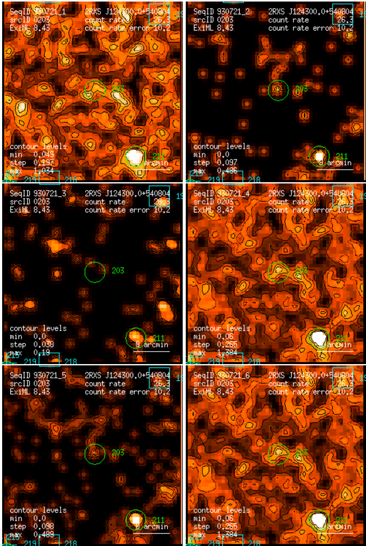
Figure 203: RASS 930721: detection 0203: band rate images, Gaussian filter: (1) PSPC channels 11 – 41, (2) 52 – 90, (3) 91 – 201, (4) 11 – 235, (5) 52 – 201, (6) 11 – 201. Broad band rates in counts/ks. Band rate contour levels in counts/ks/arcmin 2 .
