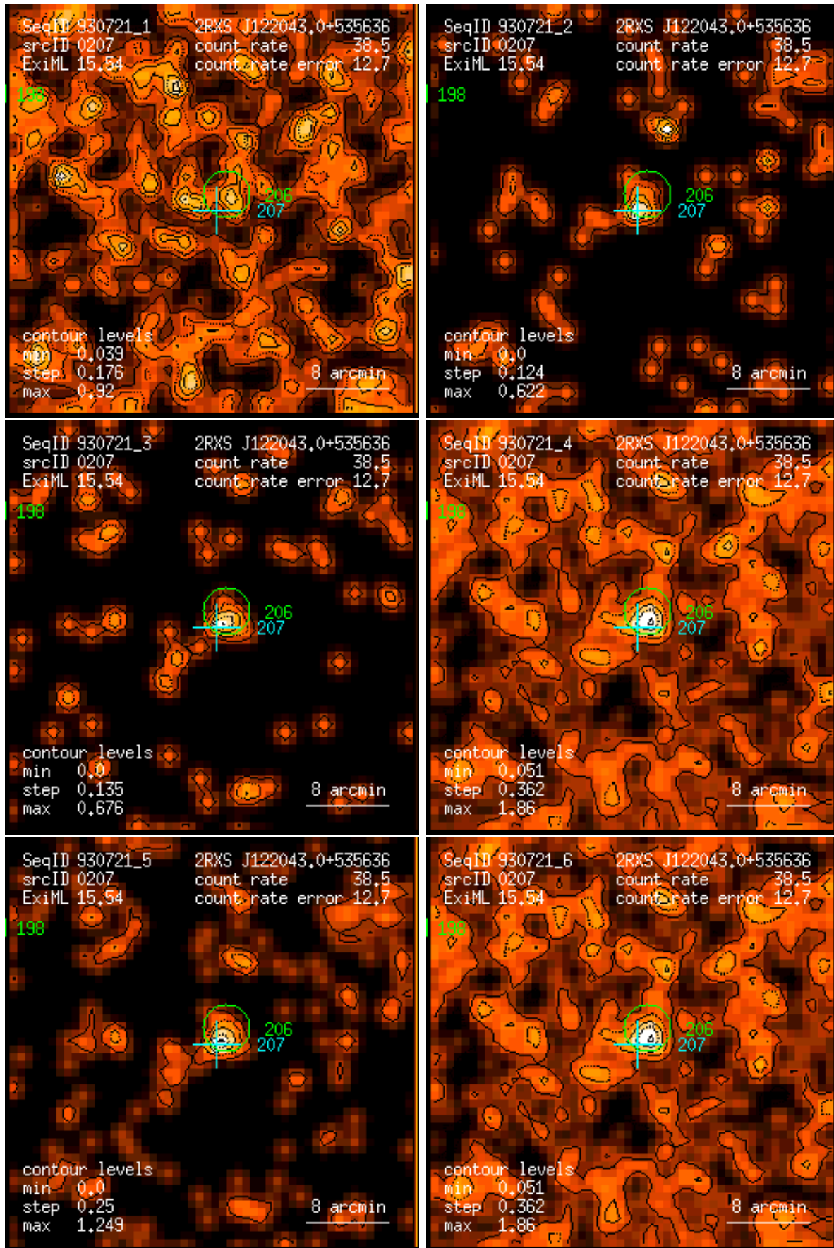
Figure 207: RASS 930721: detection 0207: band rate images, Gaussian filter: (1) PSPC channels 11 – 41, (2) 52 – 90, (3) 91 – 201, (4) 11 – 235, (5) 52 – 201, (6) 11 – 201. Broad band rates in counts/ks. Band rate contour levels in counts/ks/arcmin 2 .
