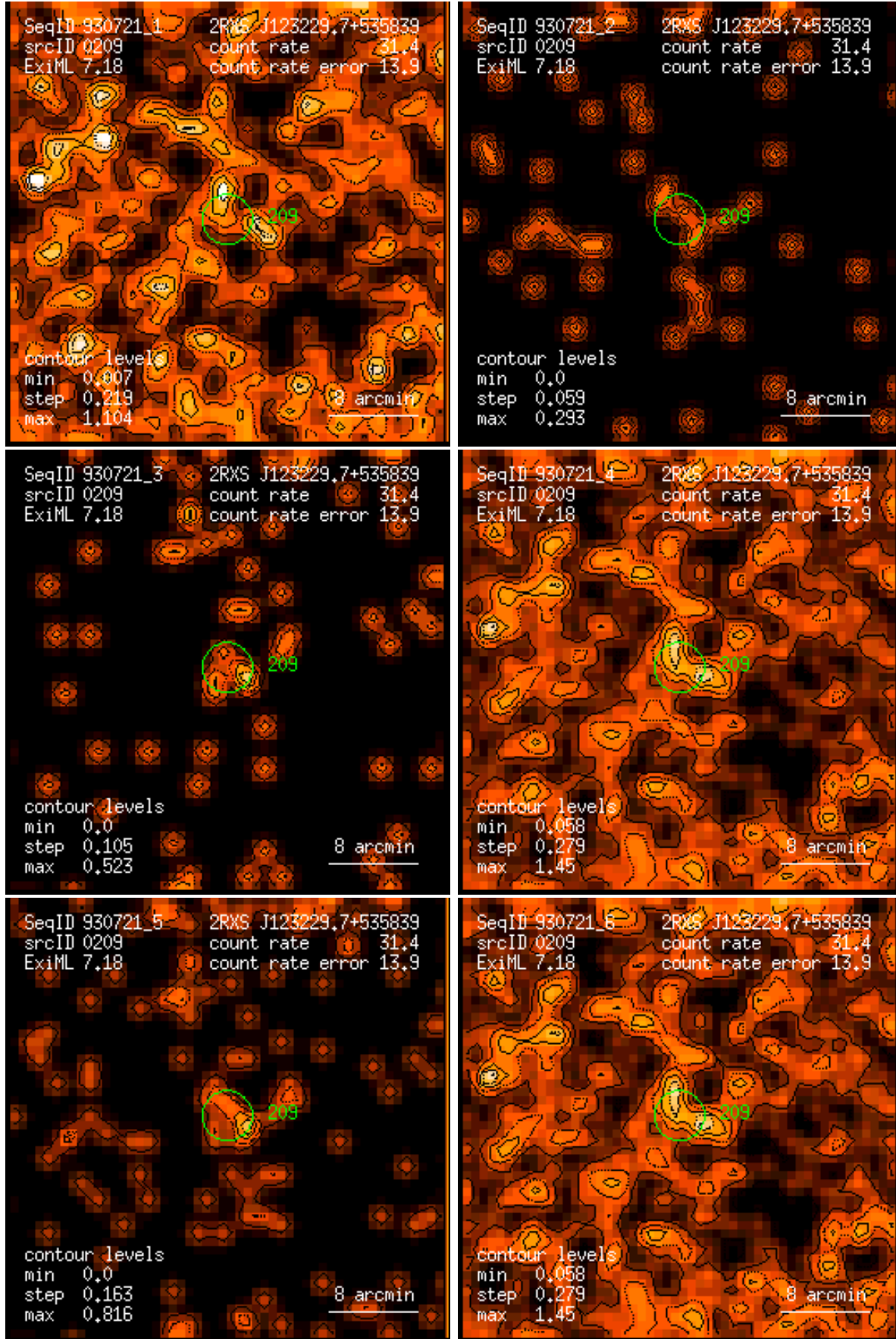
Figure 209: RASS 930721: detection 0209: band rate images, Gaussian filter: (1) PSPC channels 11 – 41, (2) 52 – 90, (3) 91 – 201, (4) 11 – 235, (5) 52 – 201, (6) 11 – 201. Broad band rates in counts/ks. Band rate contour levels in counts/ks/arcmin 2 .
