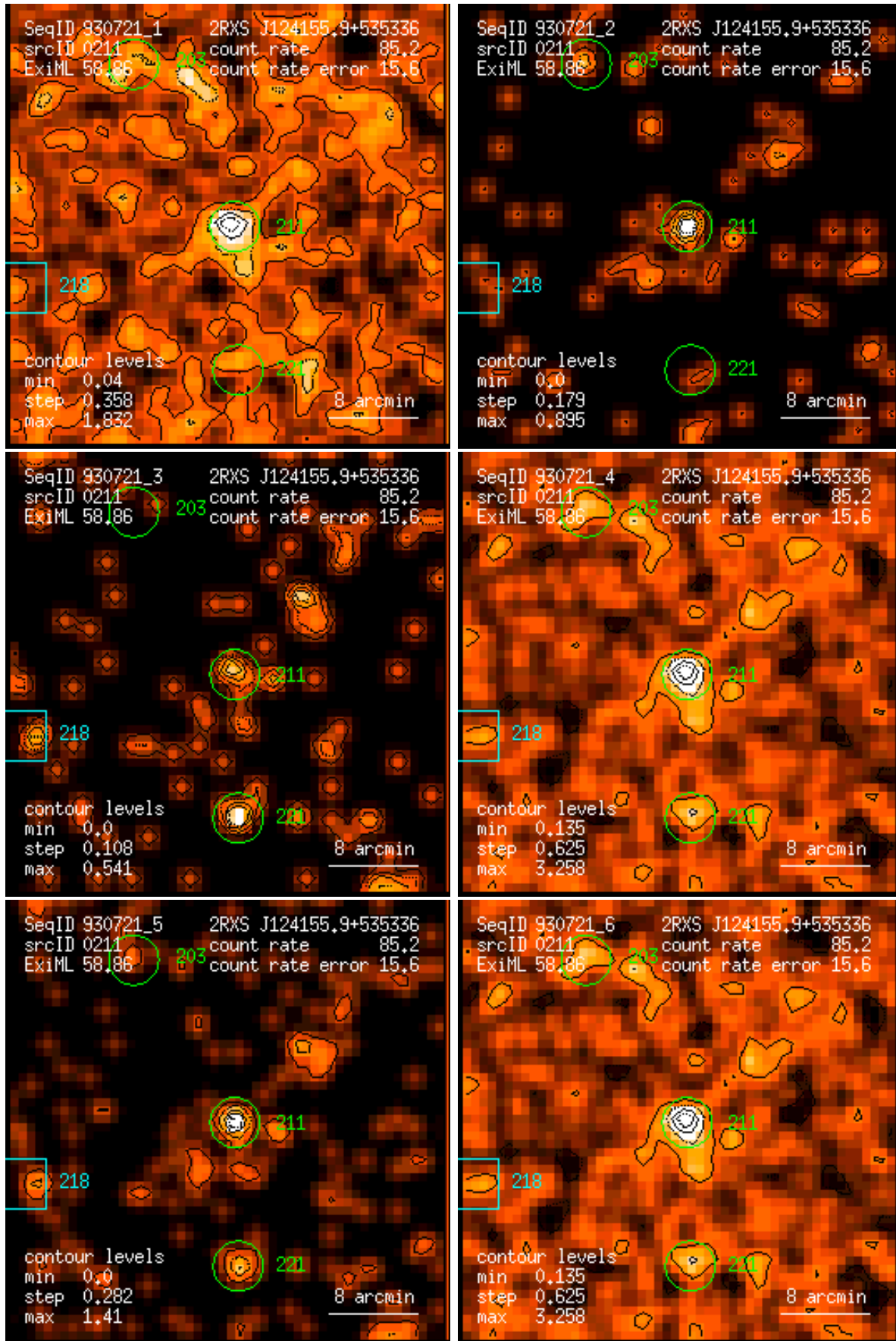
Figure 211: RASS 930721: detection 0211: band rate images, Gaussian filter: (1) PSPC channels 11 – 41, (2) 52 – 90, (3) 91 – 201, (4) 11 – 235, (5) 52 – 201, (6) 11 – 201. Broad band rates in counts/ks. Band rate contour levels in counts/ks/arcmin 2 .
