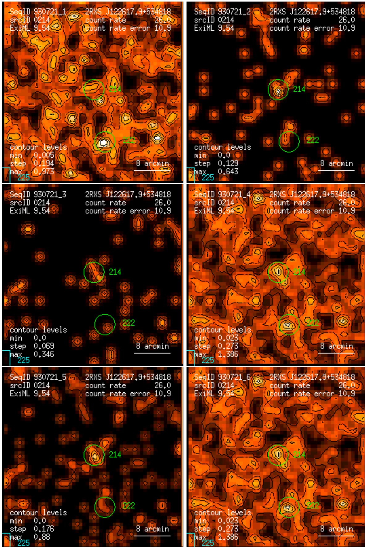
Figure 214: RASS 930721: detection 0214: band rate images, Gaussian filter: (1) PSPC channels 11 – 41, (2) 52 – 90, (3) 91 – 201, (4) 11 – 235, (5) 52 – 201, (6) 11 – 201. Broad band rates in counts/ks. Band rate contour levels in counts/ks/arcmin 2 .
