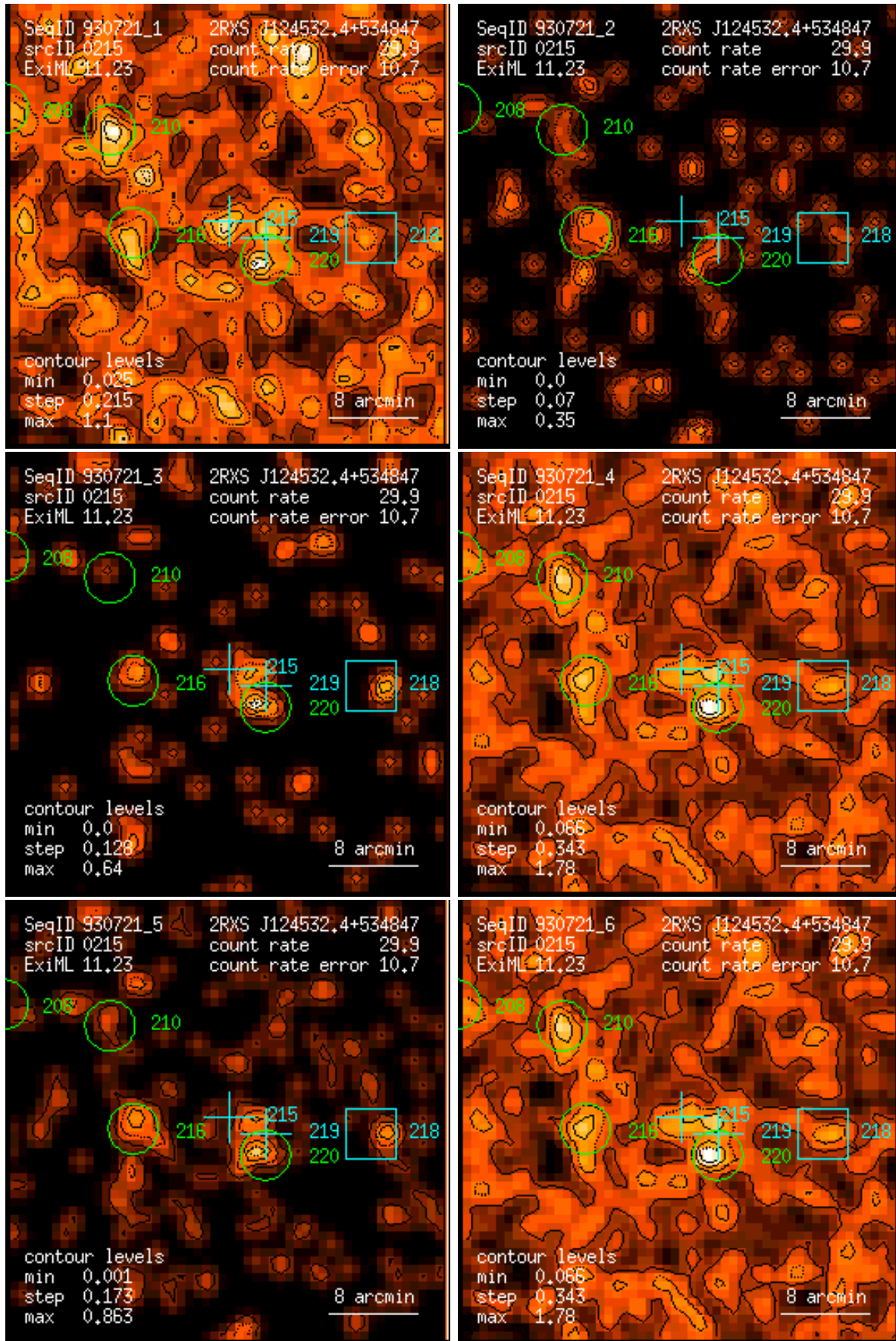
Figure 215: RASS 930721: detection 0215: band rate images, Gaussian filter: (1) PSPC channels 11 – 41, (2) 52 – 90, (3) 91 – 201, (4) 11 – 235, (5) 52 – 201, (6) 11 – 201. Broad band rates in counts/ks. Band rate contour levels in counts/ks/arcmin 2 .
