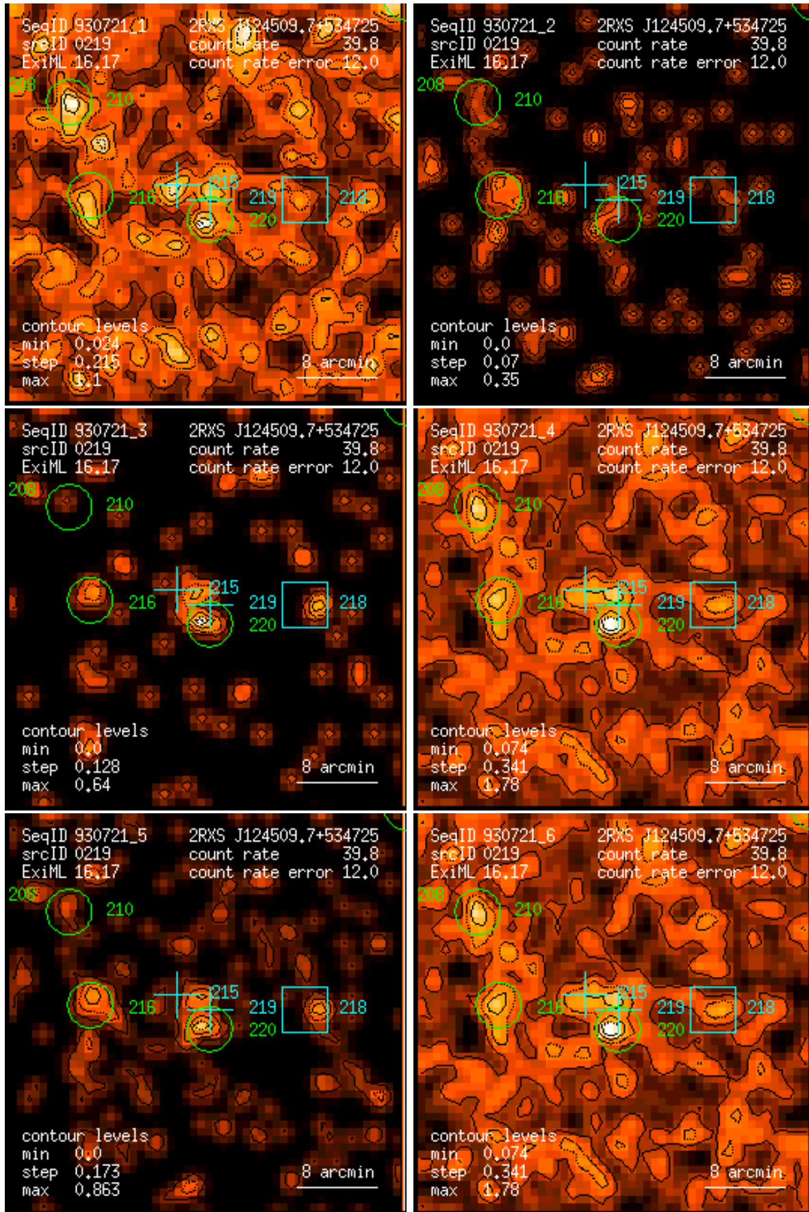
Figure 219: RASS 930721: detection 0219: band rate images, Gaussian filter: (1) PSPC channels 11 – 41, (2) 52 – 90, (3) 91 – 201, (4) 11 – 235, (5) 52 – 201, (6) 11 – 201. Broad band rates in counts/ks. Band rate contour levels in counts/ks/arcmin 2 .
