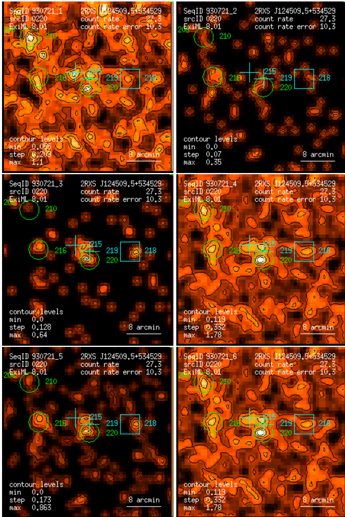
Figure 220: RASS 930721: detection 0220: band rate images, Gaussian filter: (1) PSPC channels 11 – 41, (2) 52 – 90, (3) 91 – 201, (4) 11 – 235, (5) 52 – 201, (6) 11 – 201. Broad band rates in counts/ks. Band rate contour levels in counts/ks/arcmin 2 .
