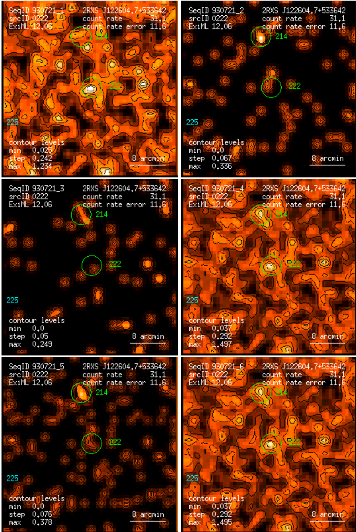
Figure 222: RASS 930721: detection 0222: band rate images, Gaussian filter: (1) PSPC channels 11 – 41, (2) 52 – 90, (3) 91 – 201, (4) 11 – 235, (5) 52 – 201, (6) 11 – 201. Broad band rates in counts/ks. Band rate contour levels in counts/ks/arcmin 2 .
