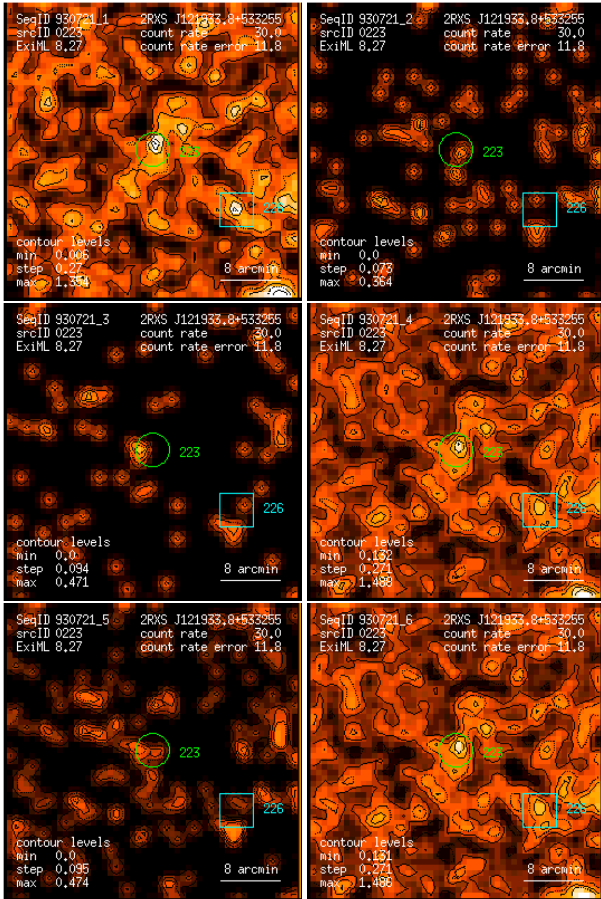
Figure 223: RASS 930721: detection 0223: band rate images, Gaussian filter: (1) PSPC channels 11 – 41, (2) 52 – 90, (3) 91 – 201, (4) 11 – 235, (5) 52 – 201, (6) 11 – 201. Broad band rates in counts/ks. Band rate contour levels in counts/ks/arcmin 2 .
