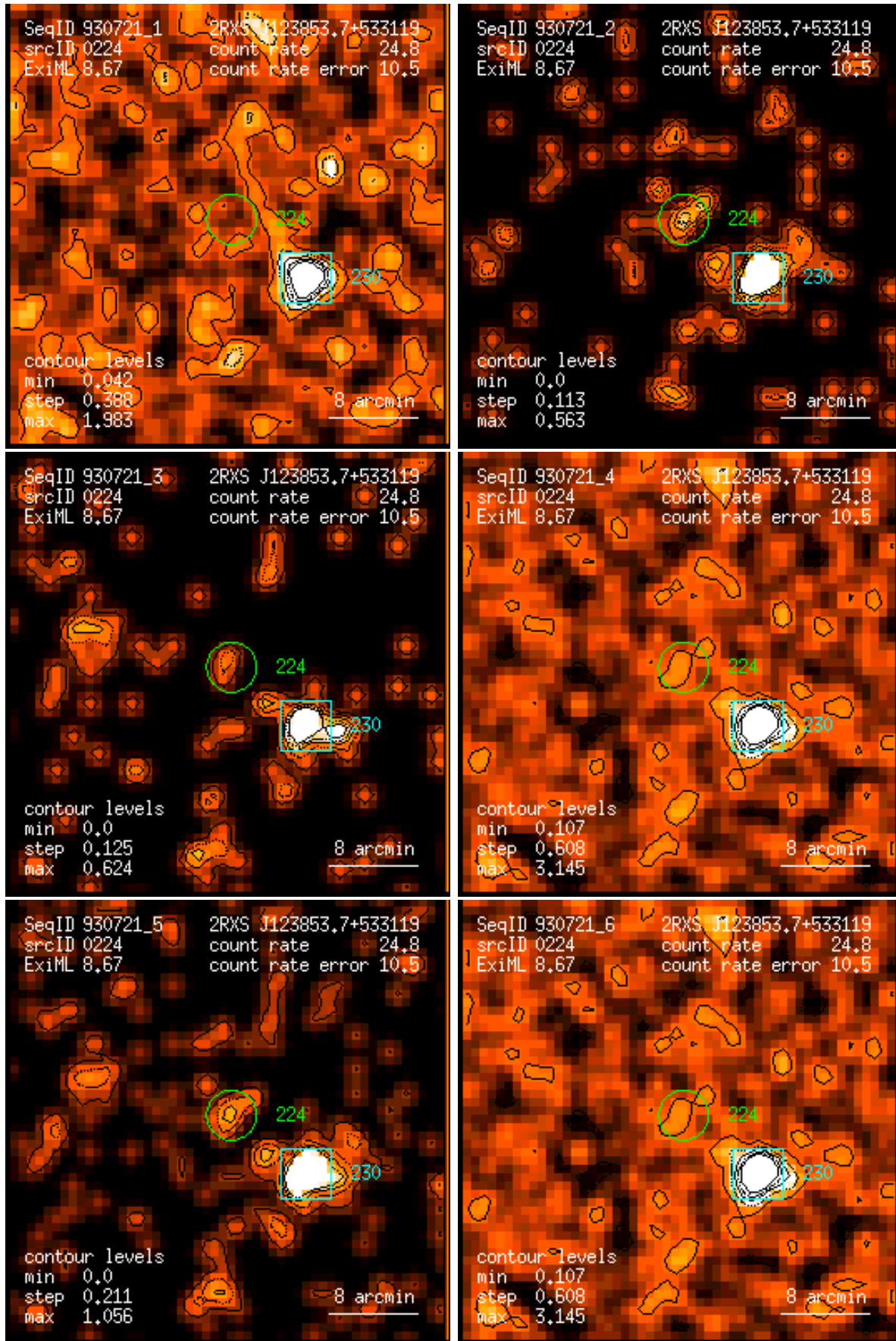
Figure 224: RASS 930721: detection 0224: band rate images, Gaussian filter: (1) PSPC channels 11 – 41, (2) 52 – 90, (3) 91 – 201, (4) 11 – 235, (5) 52 – 201, (6) 11 – 201. Broad band rates in counts/ks. Band rate contour levels in counts/ks/arcmin 2 .
