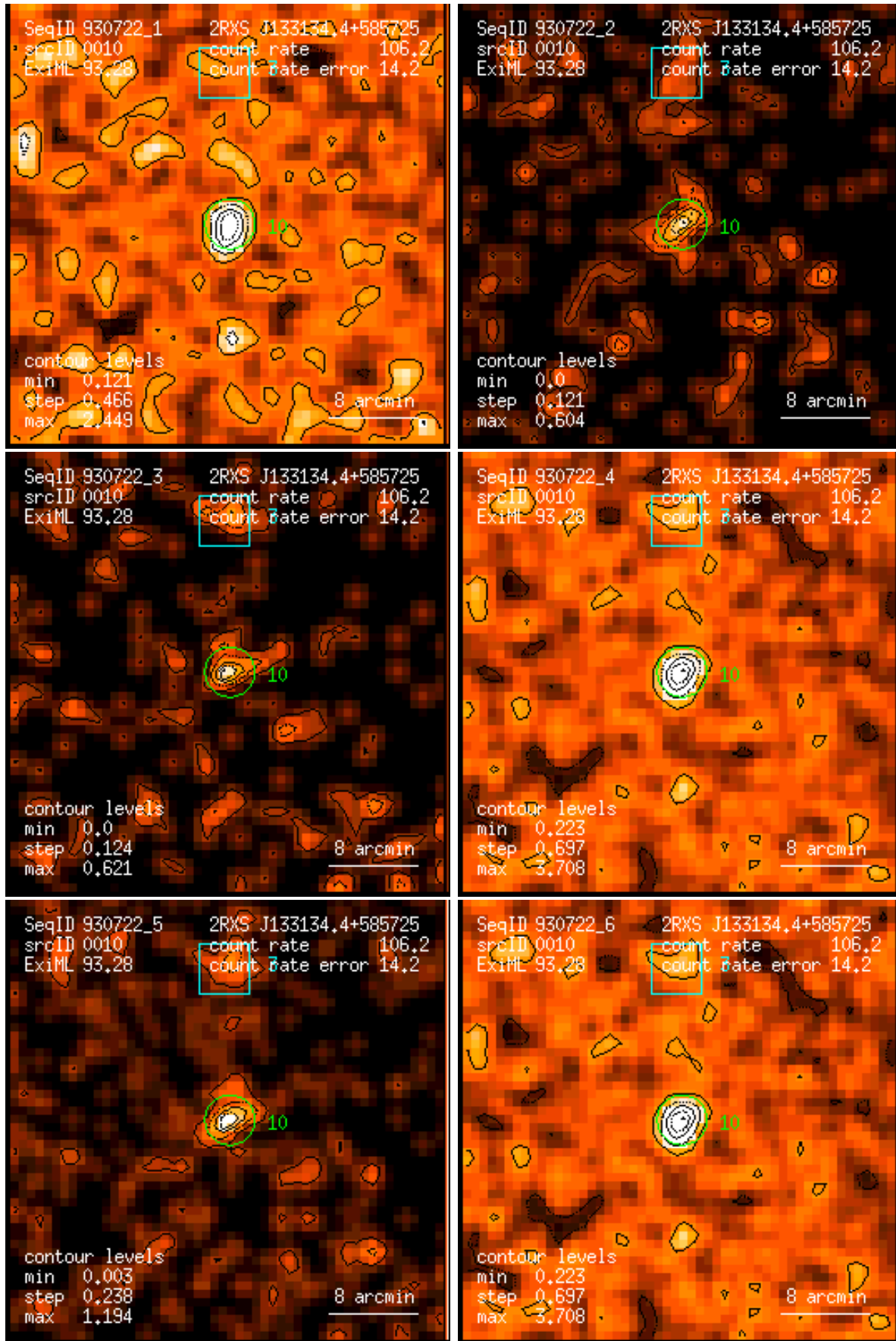
Figure 10: RASS 930722: detection 0010: band rate images, Gaussian filter: (1) PSPC channels 11 – 41, (2) 52 – 90, (3) 91 – 201, (4) 11 – 235, (5) 52 – 201, (6) 11 – 201. Broad band rates in counts/ks. Band rate contour levels in counts/ks/arcmin 2 .
