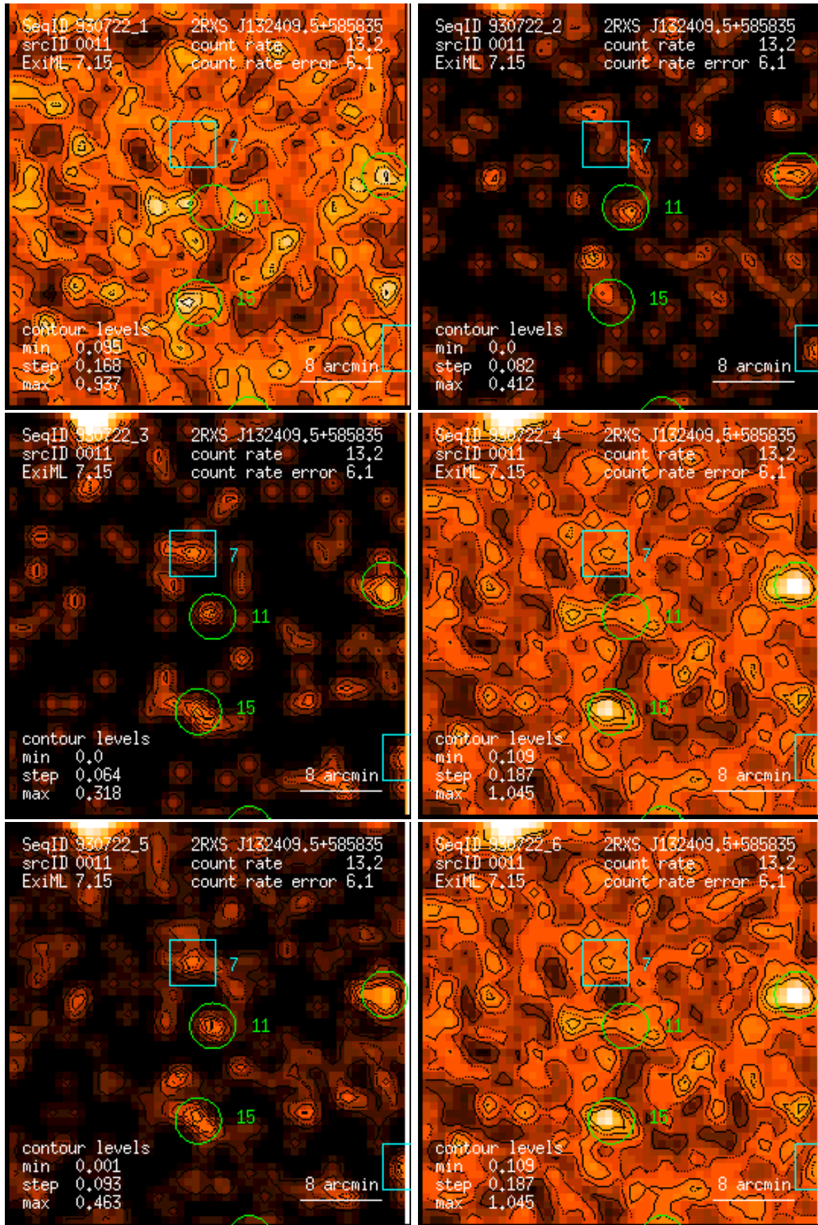
Figure 11: RASS 930722: detection 0011: band rate images, Gaussian filter: (1) PSPC channels 11 – 41, (2) 52 – 90, (3) 91 – 201, (4) 11 – 235, (5) 52 – 201, (6) 11 – 201. Broad band rates in counts/ks. Band rate contour levels in counts/ks/arcmin 2 .
