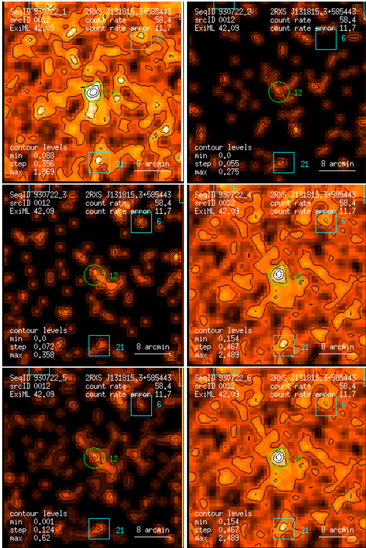
Figure 12: RASS 930722: detection 0012: band rate images, Gaussian filter: (1) PSPC channels 11 – 41, (2) 52 – 90, (3) 91 – 201, (4) 11 – 235, (5) 52 – 201, (6) 11 – 201. Broad band rates in counts/ks. Band rate contour levels in counts/ks/arcmin 2 .
