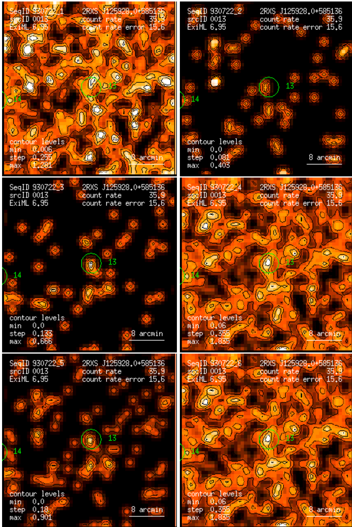
Figure 13: RASS 930722: detection 0013: band rate images, Gaussian filter: (1) PSPC channels 11 – 41, (2) 52 – 90, (3) 91 – 201, (4) 11 – 235, (5) 52 – 201, (6) 11 – 201. Broad band rates in counts/ks. Band rate contour levels in counts/ks/arcmin 2 .
