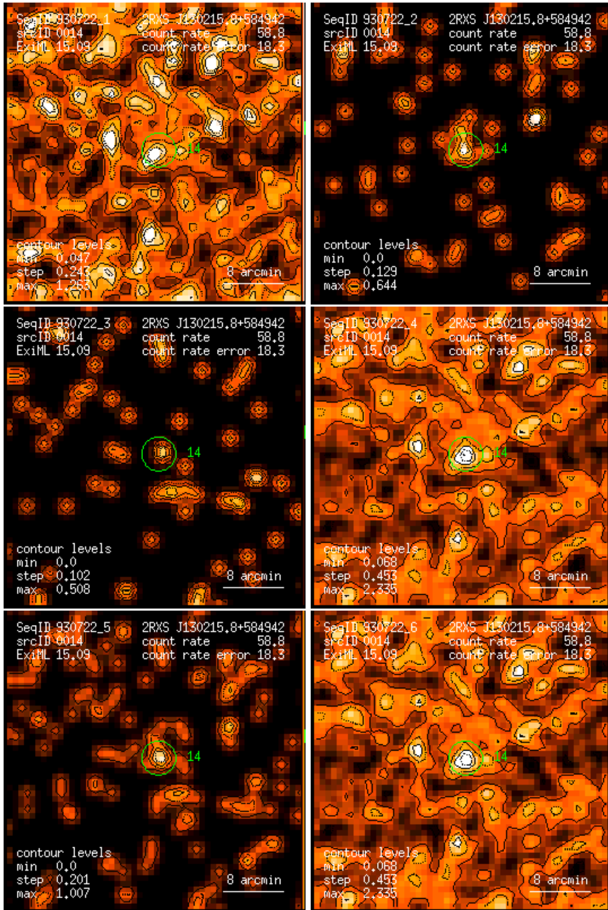
Figure 14: RASS 930722: detection 0014: band rate images, Gaussian filter: (1) PSPC channels 11 – 41, (2) 52 – 90, (3) 91 – 201, (4) 11 – 235, (5) 52 – 201, (6) 11 – 201. Broad band rates in counts/ks. Band rate contour levels in counts/ks/arcmin 2 .
