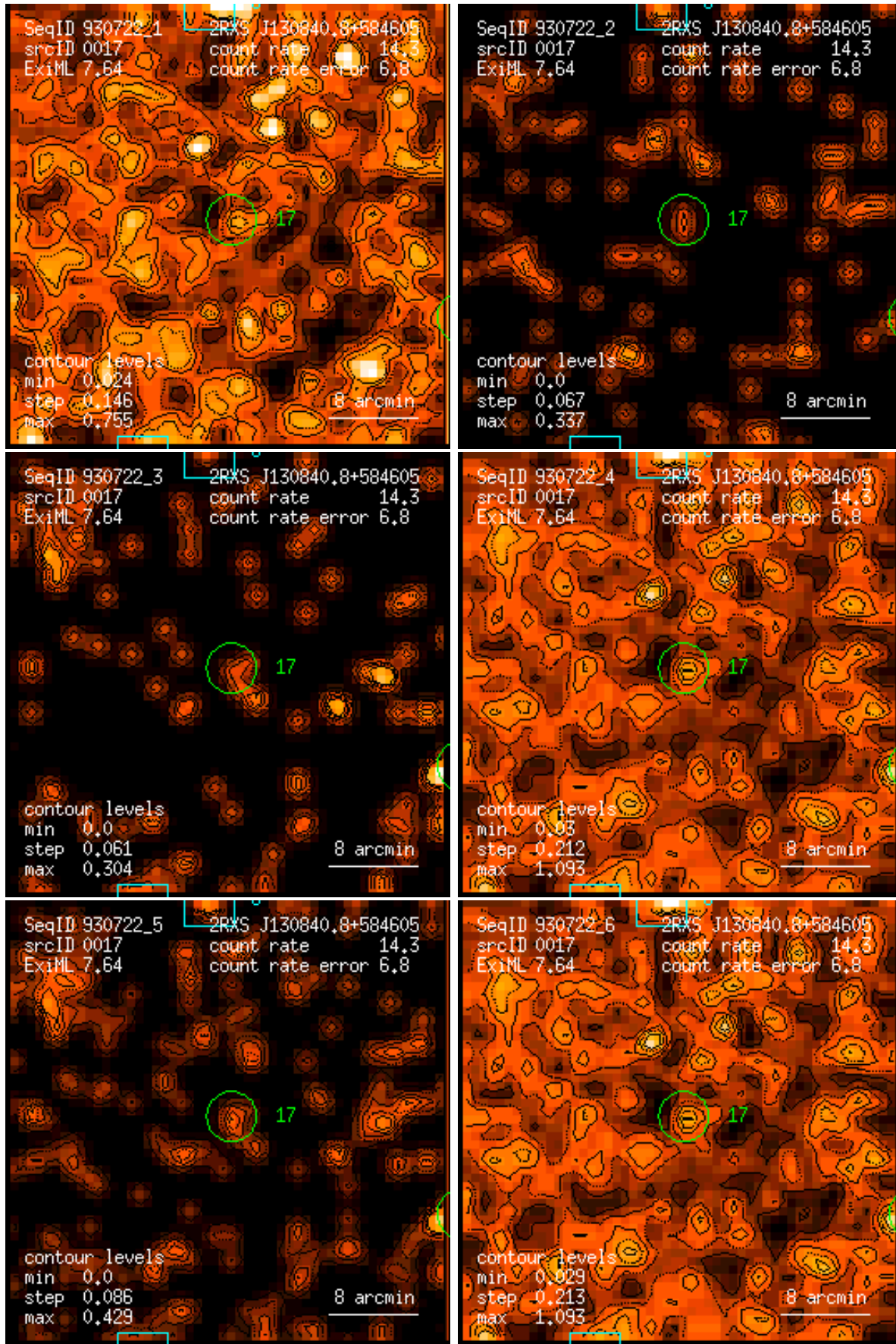
Figure 17: RASS 930722: detection 0017: band rate images, Gaussian filter: (1) PSPC channels 11 – 41, (2) 52 – 90, (3) 91 – 201, (4) 11 – 235, (5) 52 – 201, (6) 11 – 201. Broad band rates in counts/ks. Band rate contour levels in counts/ks/arcmin 2 .
