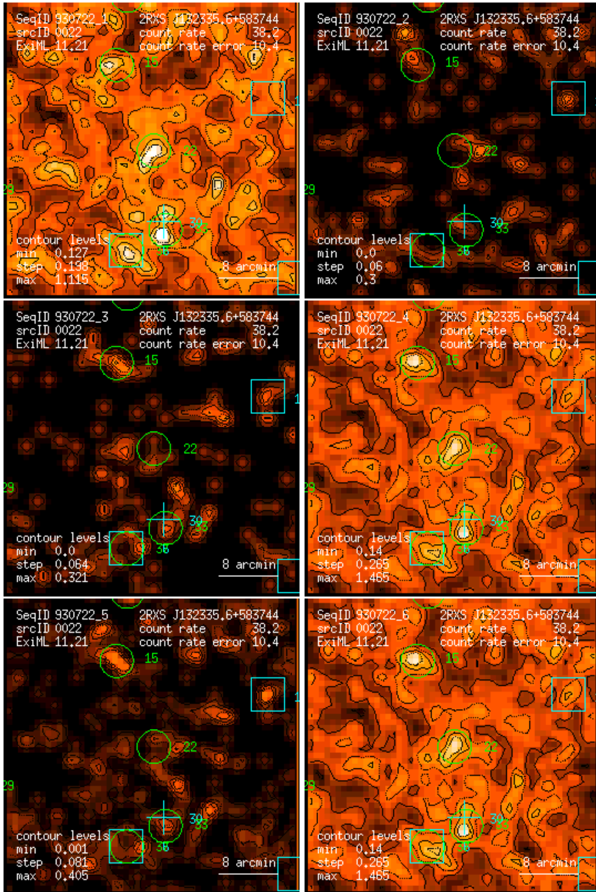
Figure 22: RASS 930722: detection 0022: band rate images, Gaussian filter: (1) PSPC channels 11 – 41, (2) 52 – 90, (3) 91 – 201, (4) 11 – 235, (5) 52 – 201, (6) 11 – 201. Broad band rates in counts/ks. Band rate contour levels in counts/ks/arcmin 2 .
