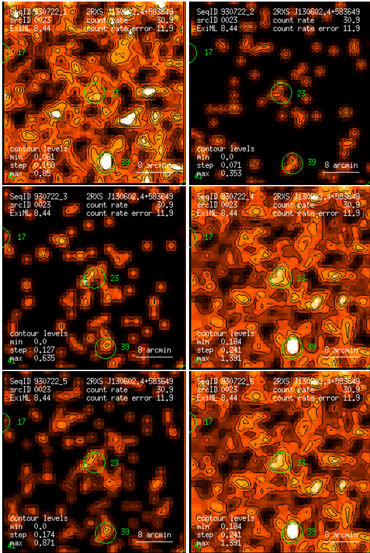
Figure 23: RASS 930722: detection 0023: band rate images, Gaussian filter: (1) PSPC channels 11 – 41, (2) 52 – 90, (3) 91 – 201, (4) 11 – 235, (5) 52 – 201, (6) 11 – 201. Broad band rates in counts/ks. Band rate contour levels in counts/ks/arcmin 2 .
