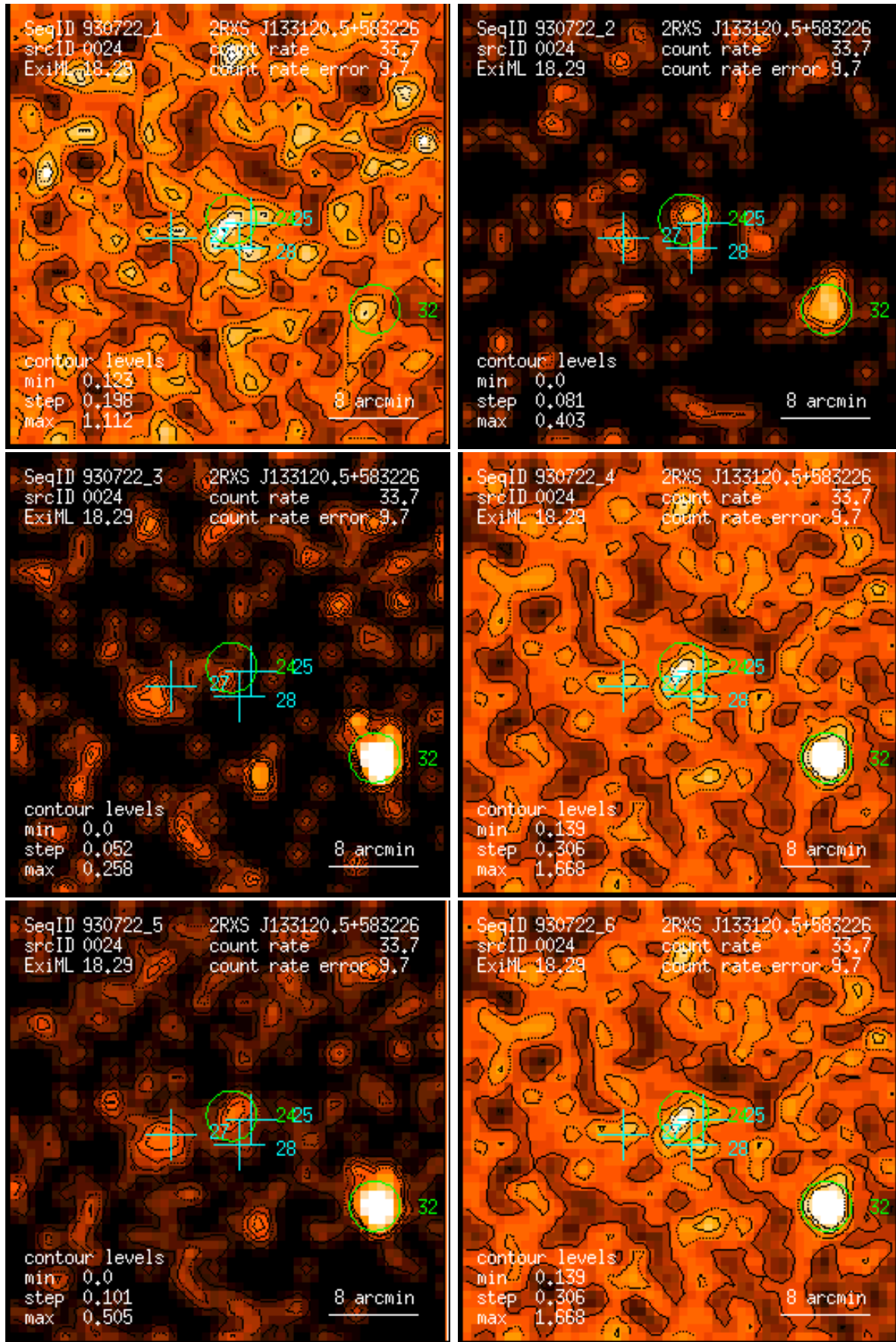
Figure 24: RASS 930722: detection 0024: band rate images, Gaussian filter: (1) PSPC channels 11 – 41, (2) 52 – 90, (3) 91 – 201, (4) 11 – 235, (5) 52 – 201, (6) 11 – 201. Broad band rates in counts/ks. Band rate contour levels in counts/ks/arcmin 2 .
