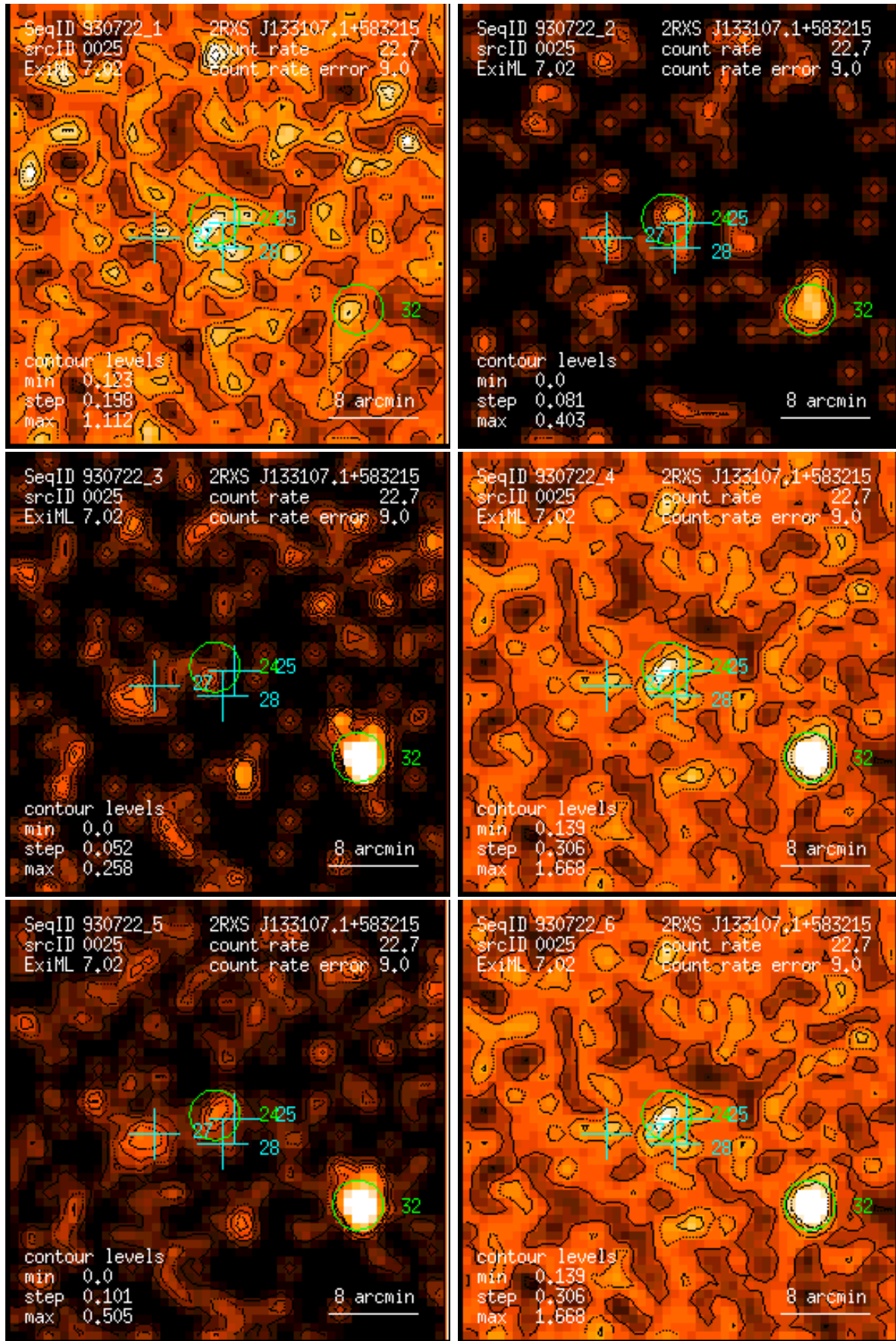
Figure 25: RASS 930722: detection 0025: band rate images, Gaussian filter: (1) PSPC channels 11 – 41, (2) 52 – 90, (3) 91 – 201, (4) 11 – 235, (5) 52 – 201, (6) 11 – 201. Broad band rates in counts/ks. Band rate contour levels in counts/ks/arcmin 2 .
