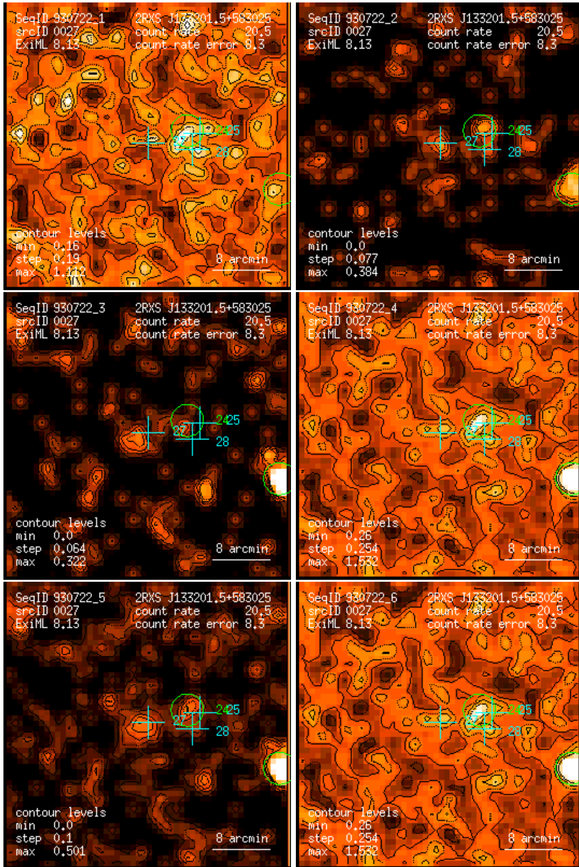
Figure 27: RASS 930722: detection 0027: band rate images, Gaussian filter: (1) PSPC channels 11 – 41, (2) 52 – 90, (3) 91 – 201, (4) 11 – 235, (5) 52 – 201, (6) 11 – 201. Broad band rates in counts/ks. Band rate contour levels in counts/ks/arcmin 2 .
