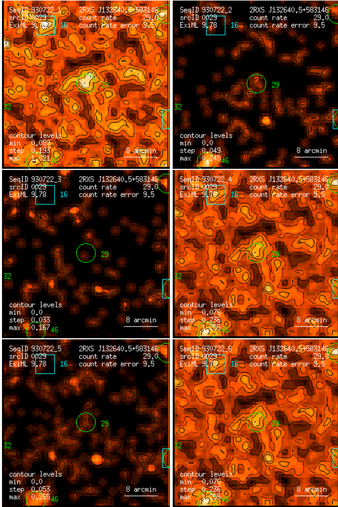
Figure 29: RASS 930722: detection 0029: band rate images, Gaussian filter: (1) PSPC channels 11 – 41, (2) 52 – 90, (3) 91 – 201, (4) 11 – 235, (5) 52 – 201, (6) 11 – 201. Broad band rates in counts/ks. Band rate contour levels in counts/ks/arcmin 2 .
