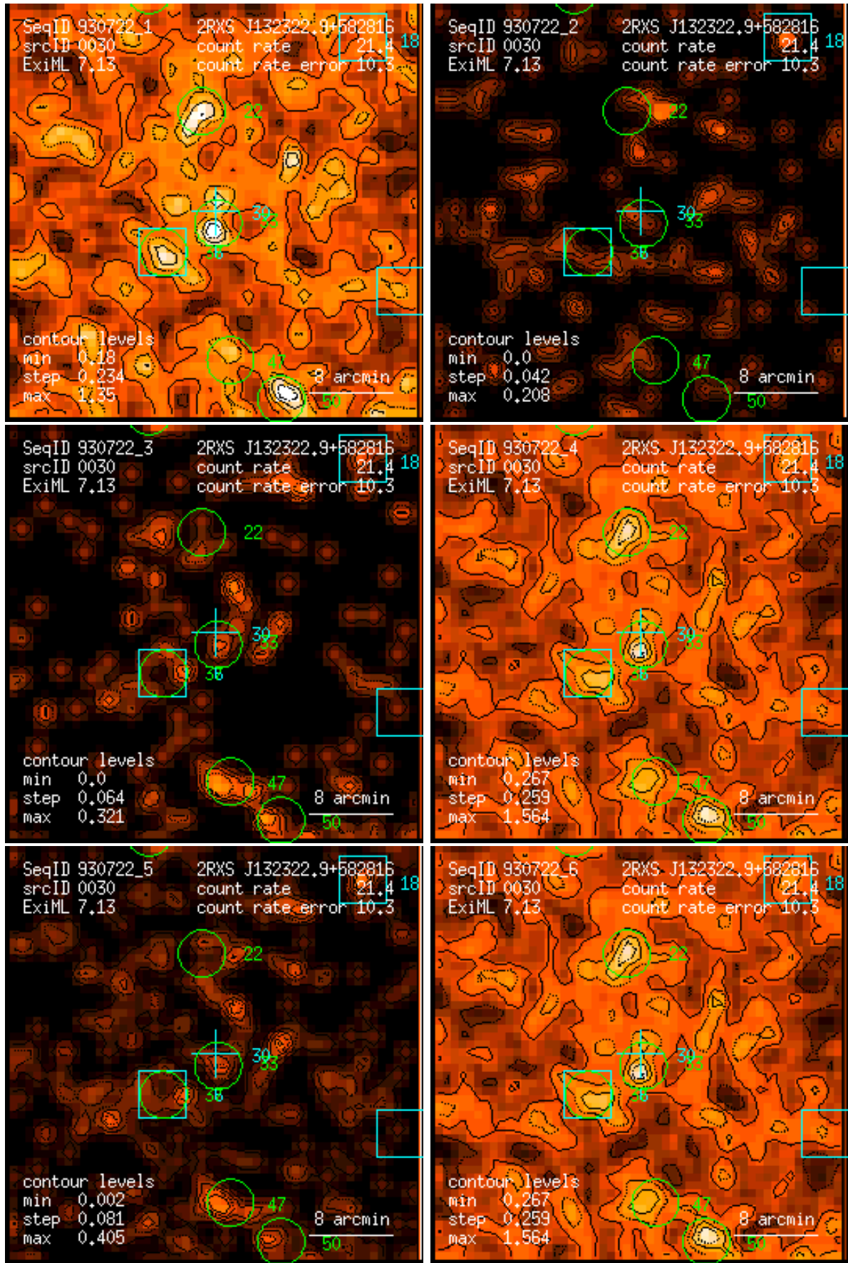
Figure 30: RASS 930722: detection 0030: band rate images, Gaussian filter: (1) PSPC channels 11 – 41, (2) 52 – 90, (3) 91 – 201, (4) 11 – 235, (5) 52 – 201, (6) 11 – 201. Broad band rates in counts/ks. Band rate contour levels in counts/ks/arcmin 2 .
