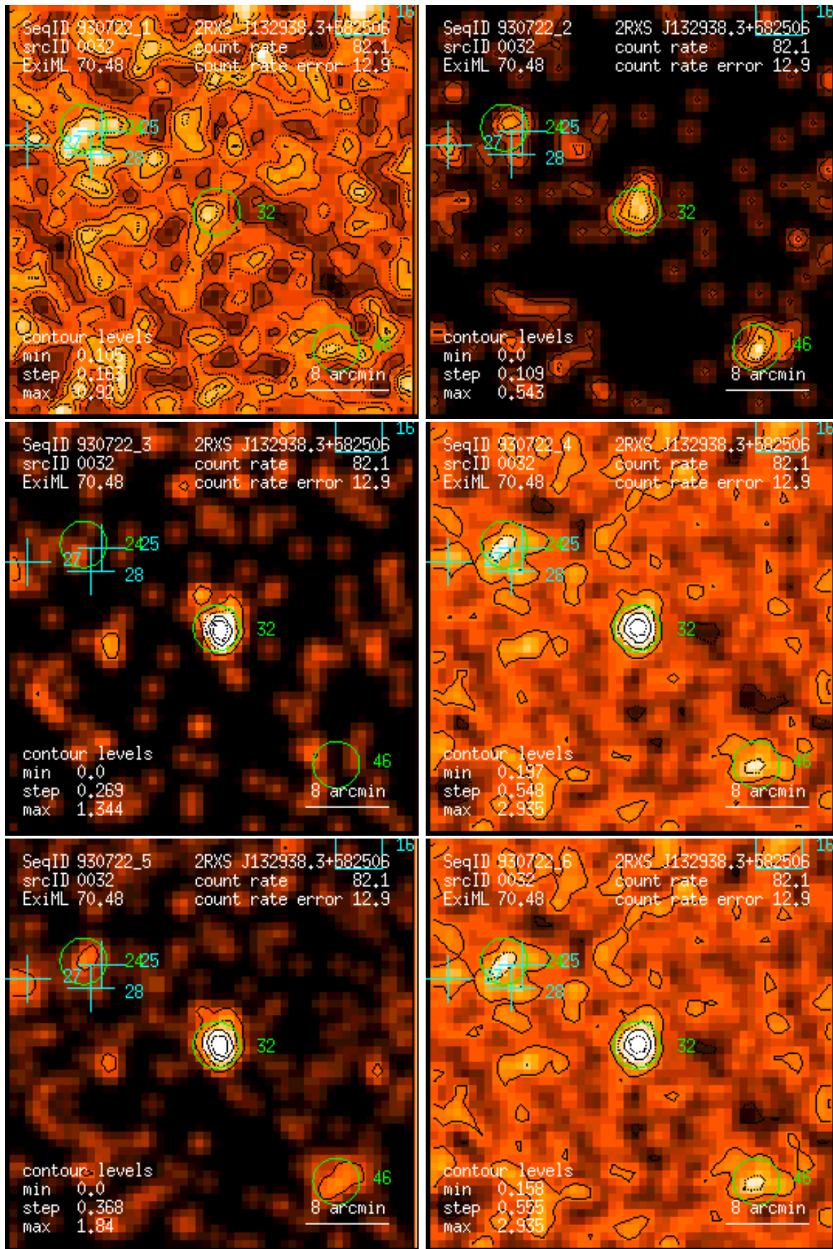
Figure 32: RASS 930722: detection 0032: band rate images, Gaussian filter: (1) PSPC channels 11 – 41, (2) 52 – 90, (3) 91 – 201, (4) 11 – 235, (5) 52 – 201, (6) 11 – 201. Broad band rates in counts/ks. Band rate contour levels in counts/ks/arcmin 2 .
