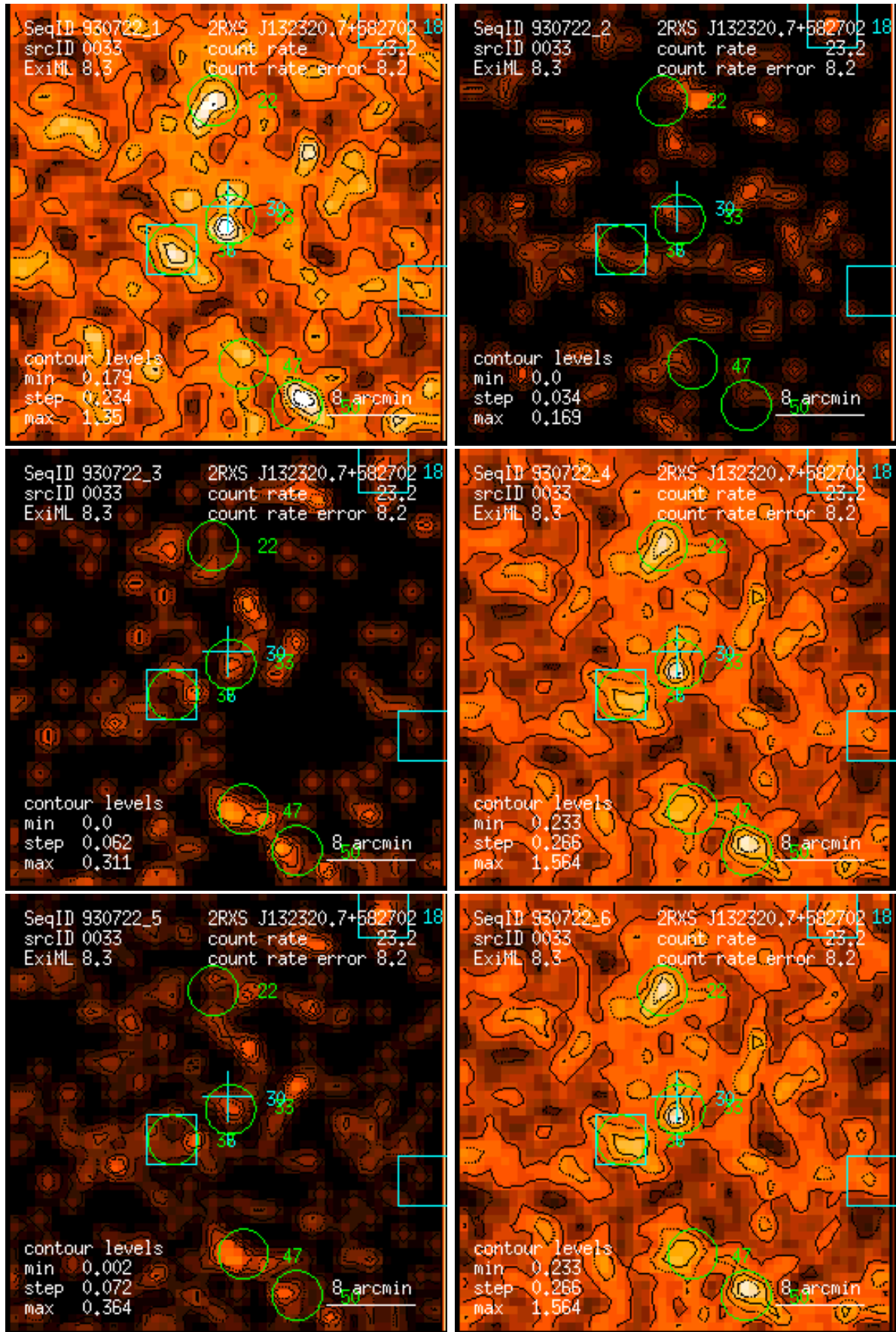
Figure 33: RASS 930722: detection 0033: band rate images, Gaussian filter: (1) PSPC channels 11 – 41, (2) 52 – 90, (3) 91 – 201, (4) 11 – 235, (5) 52 – 201, (6) 11 – 201. Broad band rates in counts/ks. Band rate contour levels in counts/ks/arcmin 2 .
