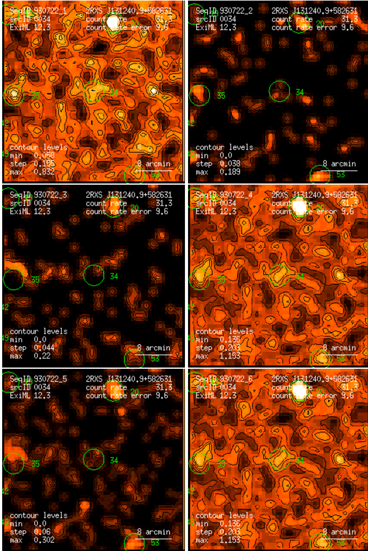
Figure 34: RASS 930722: detection 0034: band rate images, Gaussian filter: (1) PSPC channels 11 – 41, (2) 52 – 90, (3) 91 – 201, (4) 11 – 235, (5) 52 – 201, (6) 11 – 201. Broad band rates in counts/ks. Band rate contour levels in counts/ks/arcmin 2 .
