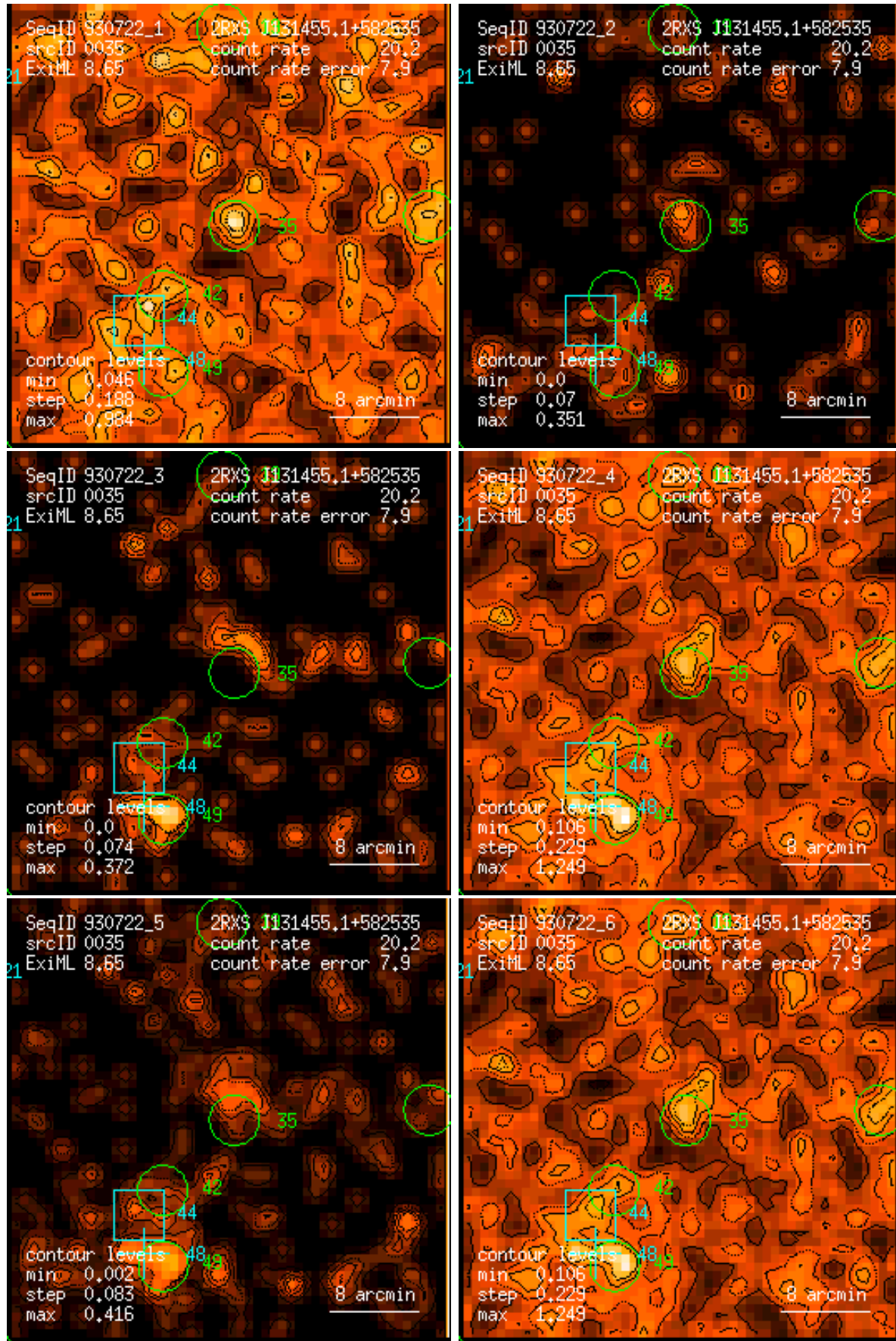
Figure 35: RASS 930722: detection 0035: band rate images, Gaussian filter: (1) PSPC channels 11 – 41, (2) 52 – 90, (3) 91 – 201, (4) 11 – 235, (5) 52 – 201, (6) 11 – 201. Broad band rates in counts/ks. Band rate contour levels in counts/ks/arcmin 2 .
