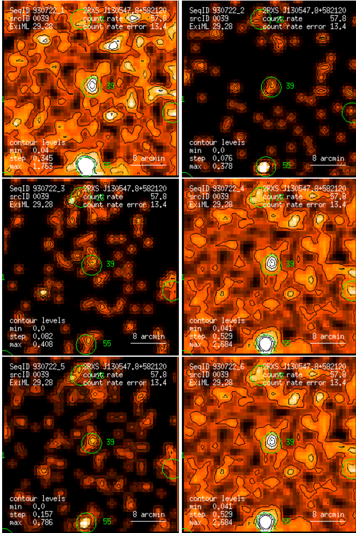
Figure 39: RASS 930722: detection 0039: band rate images, Gaussian filter: (1) PSPC channels 11 – 41, (2) 52 – 90, (3) 91 – 201, (4) 11 – 235, (5) 52 – 201, (6) 11 – 201. Broad band rates in counts/ks. Band rate contour levels in counts/ks/arcmin 2 .
