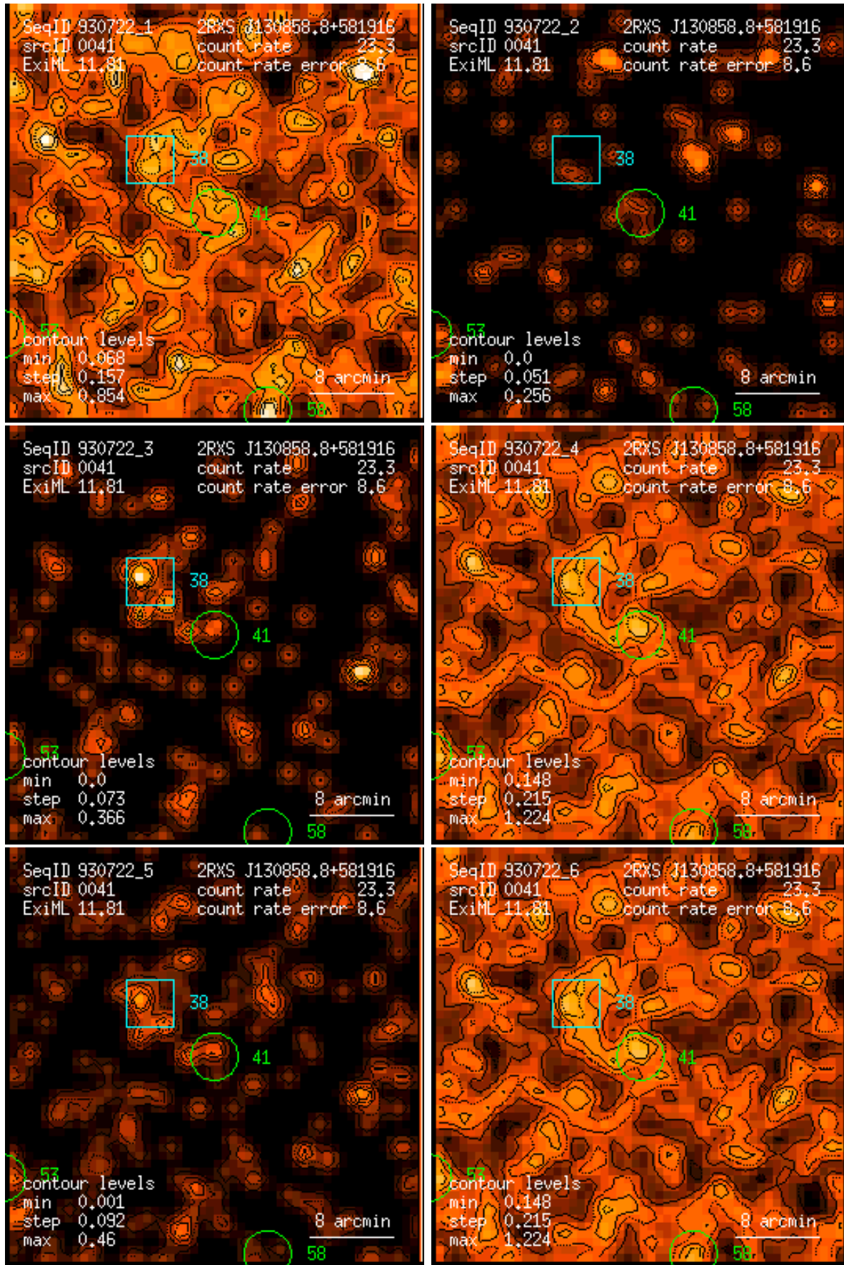
Figure 41: RASS 930722: detection 0041: band rate images, Gaussian filter: (1) PSPC channels 11 – 41, (2) 52 – 90, (3) 91 – 201, (4) 11 – 235, (5) 52 – 201, (6) 11 – 201. Broad band rates in counts/ks. Band rate contour levels in counts/ks/arcmin 2 .
