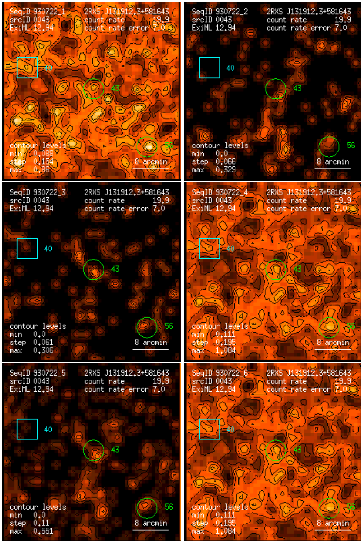
Figure 43: RASS 930722: detection 0043: band rate images, Gaussian filter: (1) PSPC channels 11 – 41, (2) 52 – 90, (3) 91 – 201, (4) 11 – 235, (5) 52 – 201, (6) 11 – 201. Broad band rates in counts/ks. Band rate contour levels in counts/ks/arcmin 2 .
