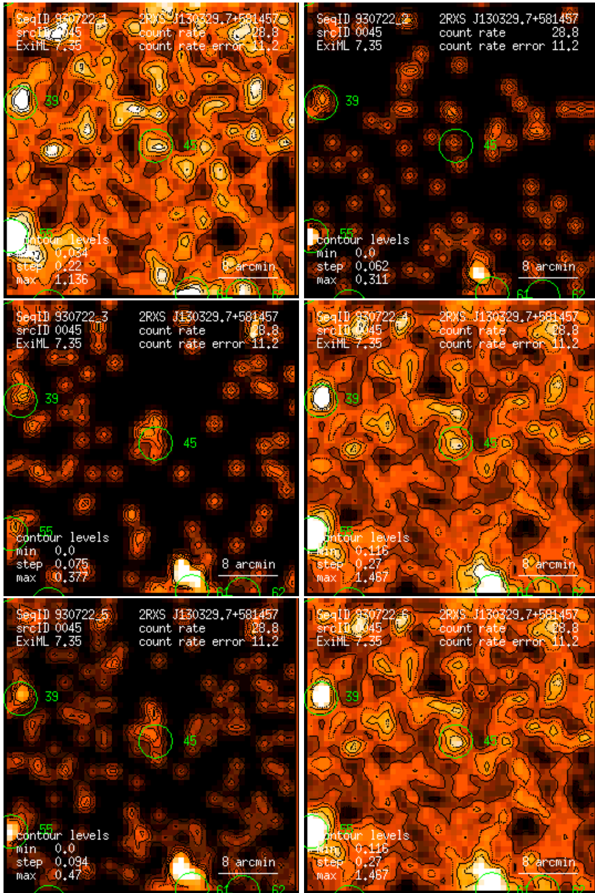
Figure 45: RASS 930722: detection 0045: band rate images, Gaussian filter: (1) PSPC channels 11 – 41, (2) 52 – 90, (3) 91 – 201, (4) 11 – 235, (5) 52 – 201, (6) 11 – 201. Broad band rates in counts/ks. Band rate contour levels in counts/ks/arcmin 2 .
