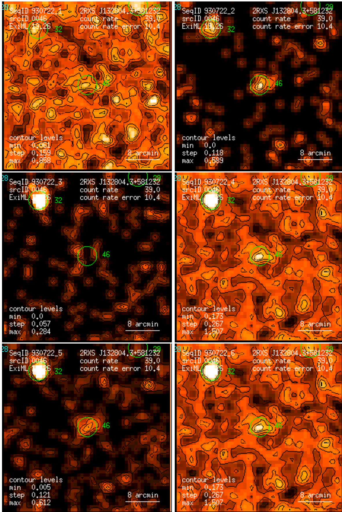
Figure 46: RASS 930722: detection 0046: band rate images, Gaussian filter: (1) PSPC channels 11 – 41, (2) 52 – 90, (3) 91 – 201, (4) 11 – 235, (5) 52 – 201, (6) 11 – 201. Broad band rates in counts/ks. Band rate contour levels in counts/ks/arcmin 2 .
