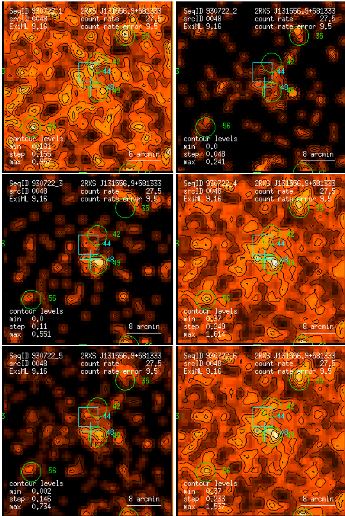
Figure 48: RASS 930722: detection 0048: band rate images, Gaussian filter: (1) PSPC channels 11 – 41, (2) 52 – 90, (3) 91 – 201, (4) 11 – 235, (5) 52 – 201, (6) 11 – 201. Broad band rates in counts/ks. Band rate contour levels in counts/ks/arcmin 2 .
