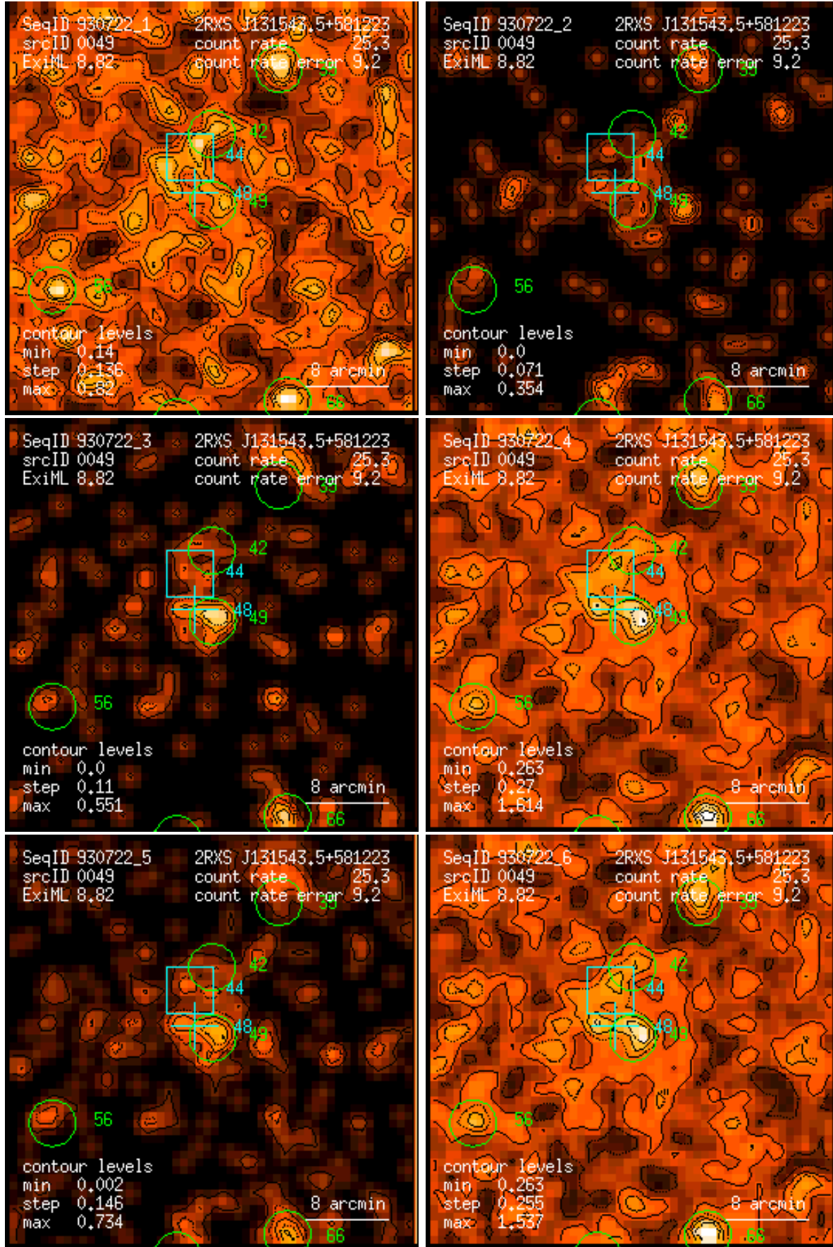
Figure 49: RASS 930722: detection 0049: band rate images, Gaussian filter: (1) PSPC channels 11 – 41, (2) 52 – 90, (3) 91 – 201, (4) 11 – 235, (5) 52 – 201, (6) 11 – 201. Broad band rates in counts/ks. Band rate contour levels in counts/ks/arcmin 2 .
