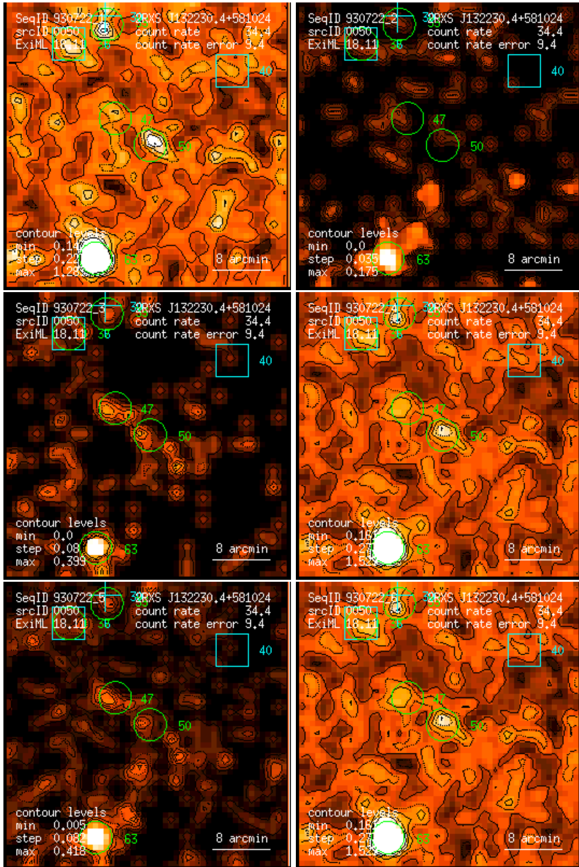
Figure 50: RASS 930722: detection 0050: band rate images, Gaussian filter: (1) PSPC channels 11 – 41, (2) 52 – 90, (3) 91 – 201, (4) 11 – 235, (5) 52 – 201, (6) 11 – 201. Broad band rates in counts/ks. Band rate contour levels in counts/ks/arcmin 2 .
