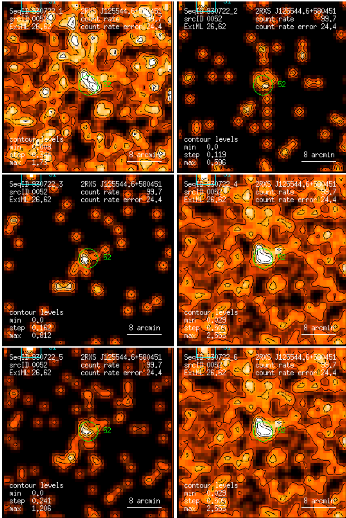
Figure 52: RASS 930722: detection 0052: band rate images, Gaussian filter: (1) PSPC channels 11 – 41, (2) 52 – 90, (3) 91 – 201, (4) 11 – 235, (5) 52 – 201, (6) 11 – 201. Broad band rates in counts/ks. Band rate contour levels in counts/ks/arcmin 2 .
