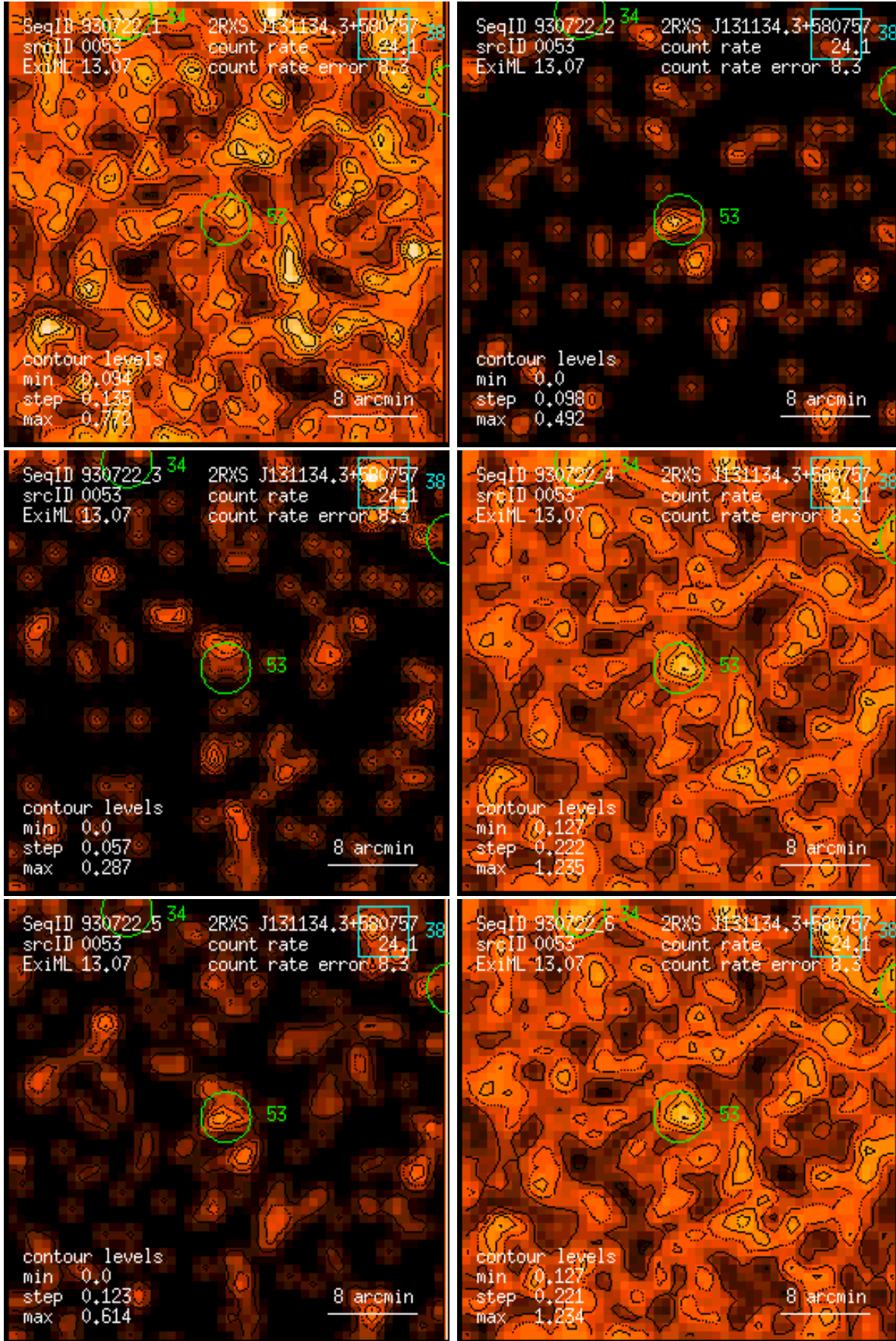
Figure 53: RASS 930722: detection 0053: band rate images, Gaussian filter: (1) PSPC channels 11 – 41, (2) 52 – 90, (3) 91 – 201, (4) 11 – 235, (5) 52 – 201, (6) 11 – 201. Broad band rates in counts/ks. Band rate contour levels in counts/ks/arcmin 2 .
