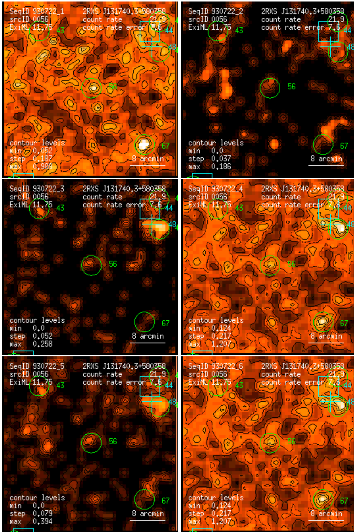
Figure 56: RASS 930722: detection 0056: band rate images, Gaussian filter: (1) PSPC channels 11 – 41, (2) 52 – 90, (3) 91 – 201, (4) 11 – 235, (5) 52 – 201, (6) 11 – 201. Broad band rates in counts/ks. Band rate contour levels in counts/ks/arcmin 2 .
