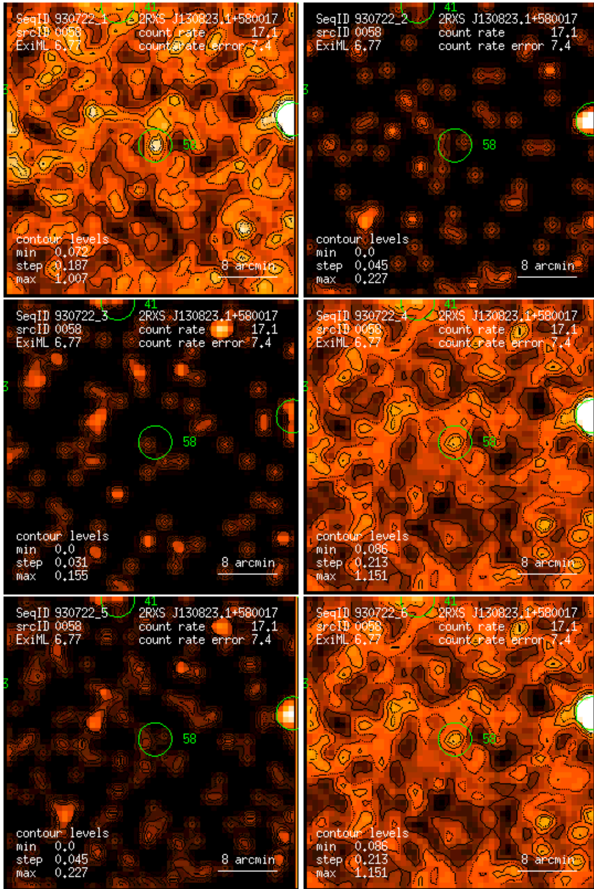
Figure 58: RASS 930722: detection 0058: band rate images, Gaussian filter: (1) PSPC channels 11 – 41, (2) 52 – 90, (3) 91 – 201, (4) 11 – 235, (5) 52 – 201, (6) 11 – 201. Broad band rates in counts/ks. Band rate contour levels in counts/ks/arcmin 2 .
