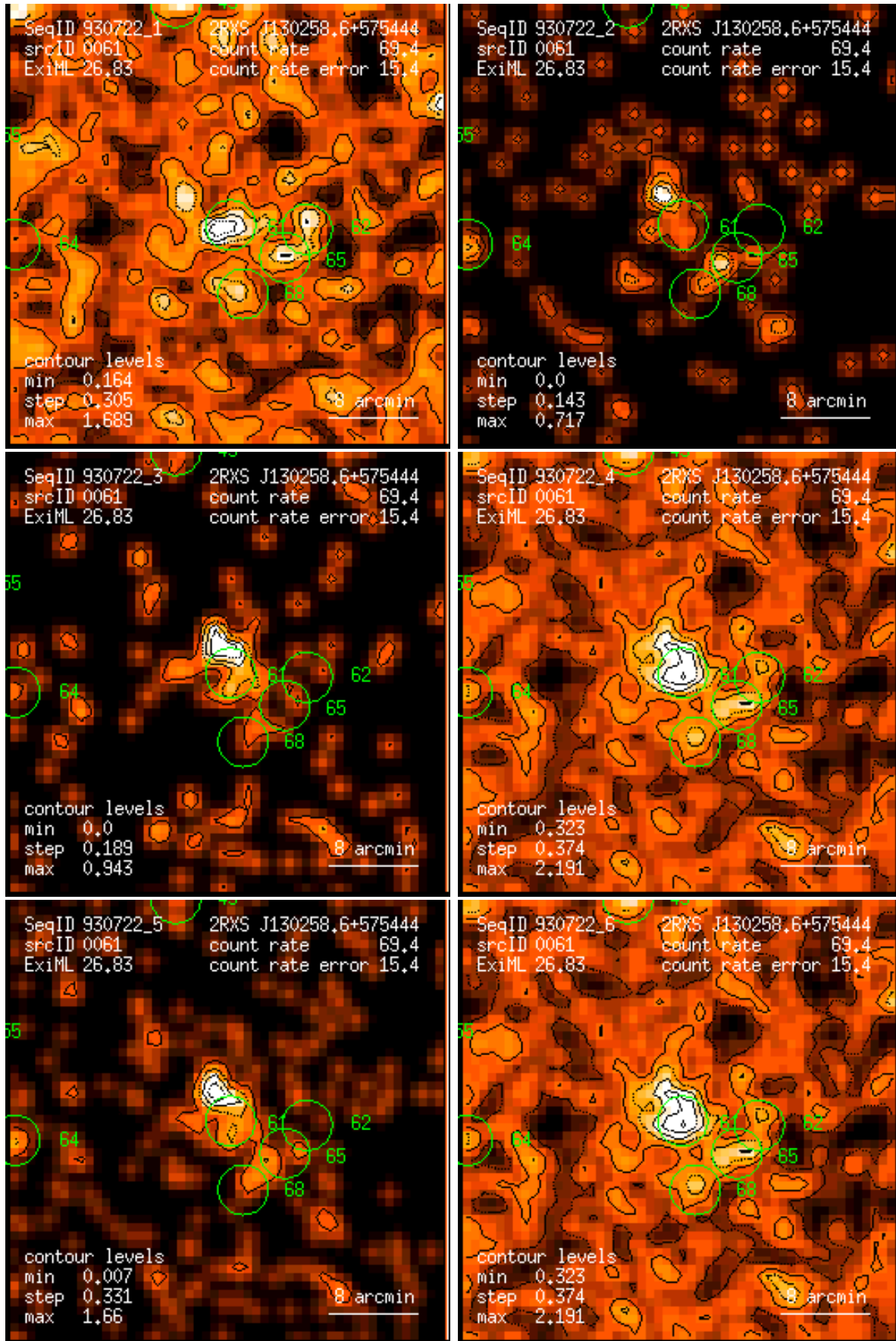
Figure 61: RASS 930722: detection 0061: band rate images, Gaussian filter: (1) PSPC channels 11 – 41, (2) 52 – 90, (3) 91 – 201, (4) 11 – 235, (5) 52 – 201, (6) 11 – 201. Broad band rates in counts/ks. Band rate contour levels in counts/ks/arcmin 2 .
