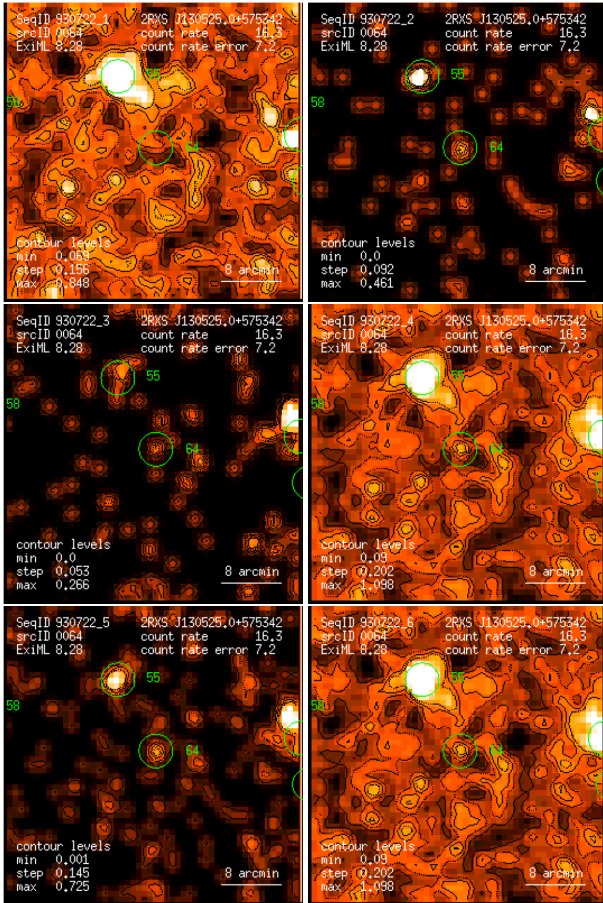
Figure 64: RASS 930722: detection 0064: band rate images, Gaussian filter: (1) PSPC channels 11 – 41, (2) 52 – 90, (3) 91 – 201, (4) 11 – 235, (5) 52 – 201, (6) 11 – 201. Broad band rates in counts/ks. Band rate contour levels in counts/ks/arcmin 2 .
