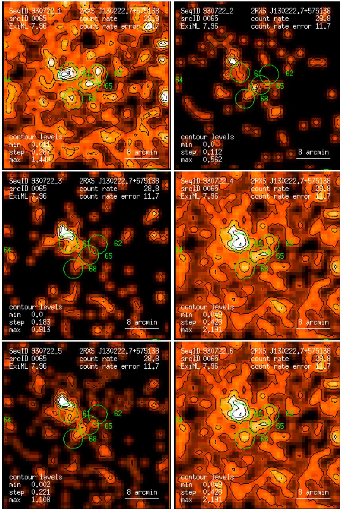
Figure 65: RASS 930722: detection 0065: band rate images, Gaussian filter: (1) PSPC channels 11 – 41, (2) 52 – 90, (3) 91 – 201, (4) 11 – 235, (5) 52 – 201, (6) 11 – 201. Broad band rates in counts/ks. Band rate contour levels in counts/ks/arcmin 2 .
