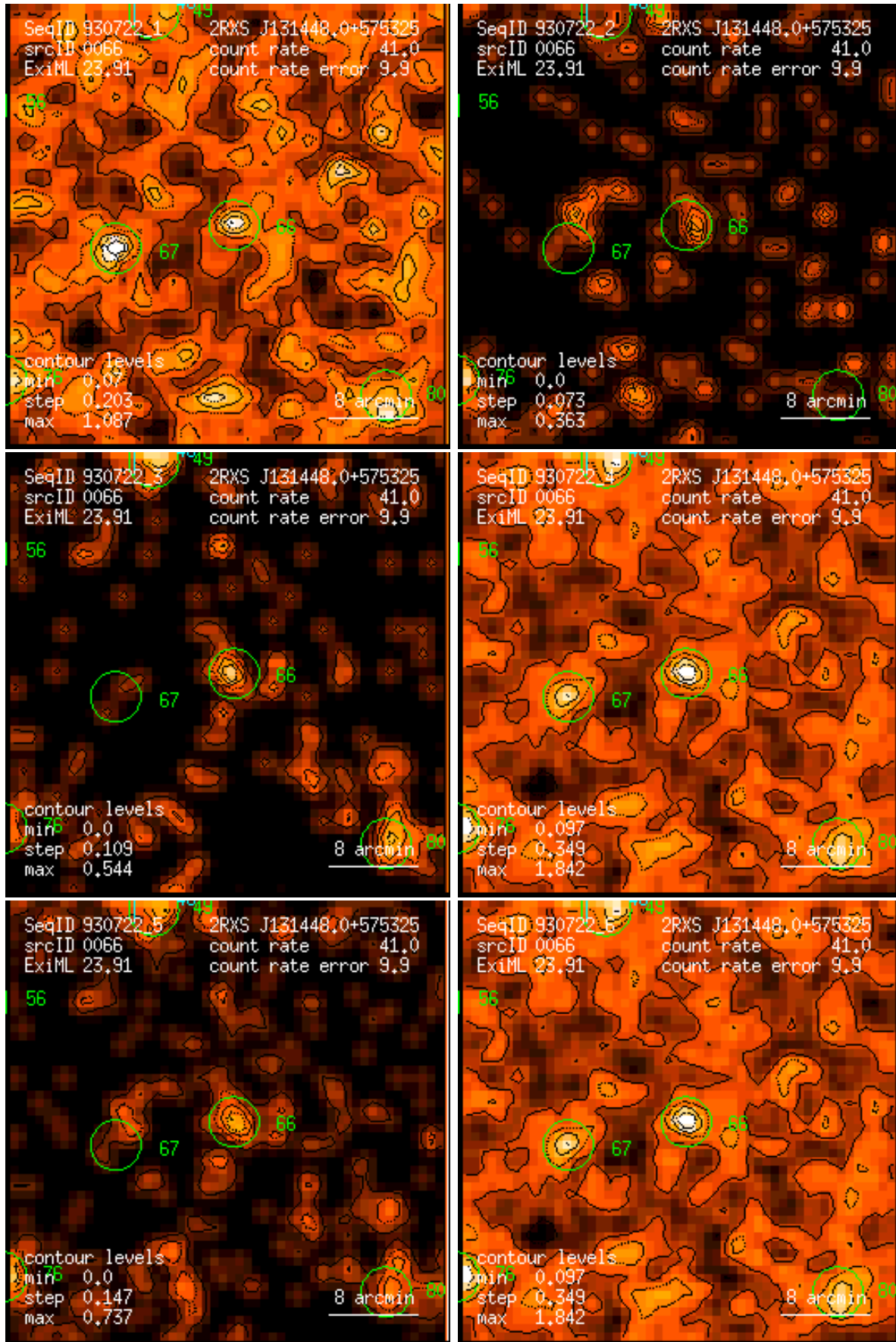
Figure 66: RASS 930722: detection 0066: band rate images, Gaussian filter: (1) PSPC channels 11 – 41, (2) 52 – 90, (3) 91 – 201, (4) 11 – 235, (5) 52 – 201, (6) 11 – 201. Broad band rates in counts/ks. Band rate contour levels in counts/ks/arcmin 2 .
