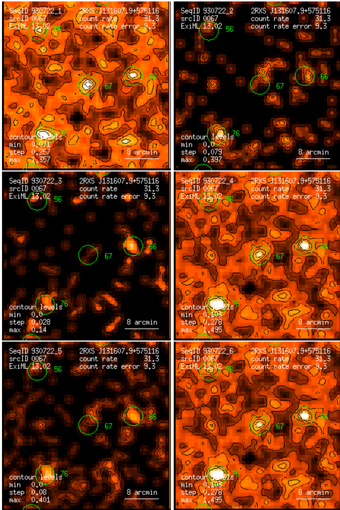
Figure 67: RASS 930722: detection 0067: band rate images, Gaussian filter: (1) PSPC channels 11 – 41, (2) 52 – 90, (3) 91 – 201, (4) 11 – 235, (5) 52 – 201, (6) 11 – 201. Broad band rates in counts/ks. Band rate contour levels in counts/ks/arcmin 2 .
